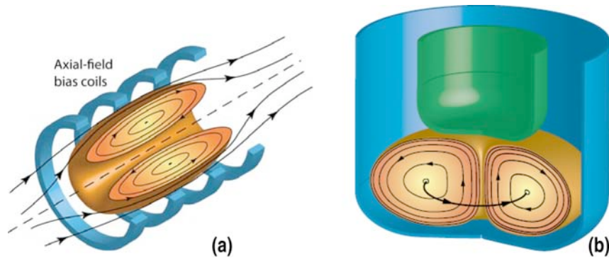
Fig. 2-5. (a) Field-reversed configuration, (b) spheromak configuration
