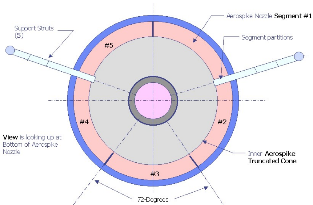
Figure 28. Nuclear DC-X/LANTR SSTO Heavy Cargo Lifter (March, 2001)
