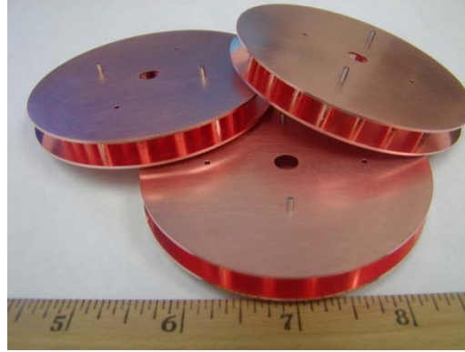
Figure 4: The 11.7 GHz PBG cells ready for tuning and brazing.
