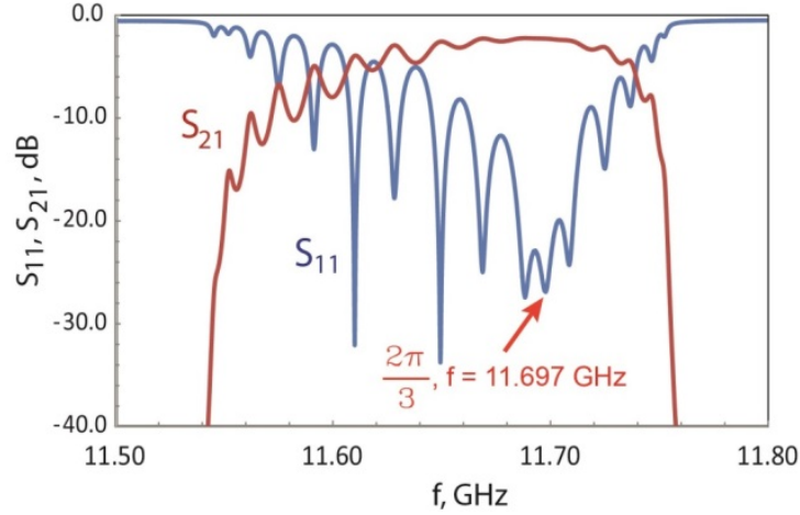
Figure 8: Transmission and reflection in the tuned 16-cell PBG structure.
