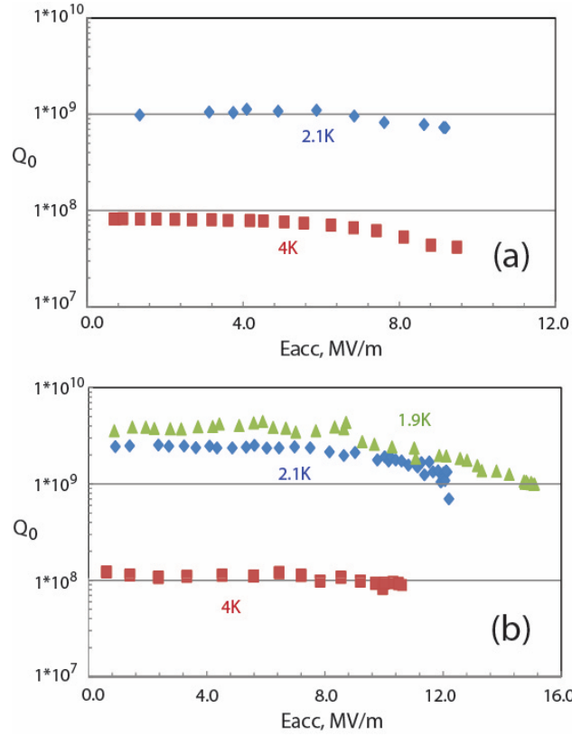
Figure 5: Unloaded qualify factor ( Q_0 ) as a function of accelerating gradient ( E_{acc} ) off the 2.1 GHz SRF PBG cavities: (a) cavity #1 tested on 3/30/12, and (b) cavity #2 tested on 4/27/12.
