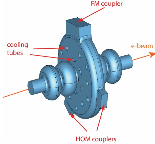
Figure 6: The 5-cell 2.1 GHz SRF accelerating module with a PBG coupling cavity.
