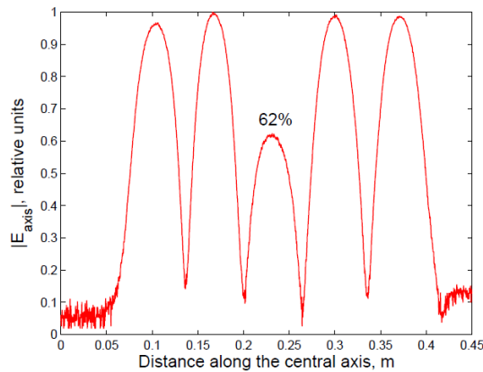
Figure 18: Magnitude of the electric field measured along the axis of the 2.1 GHz 5-cell SRF accelerating module after the tuning.
