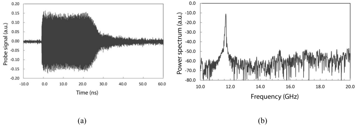
Figure 13: The rf signal in the downstream coupling waveguide of the PBG structure: (a) time-domain; (b) Fourier transform.
