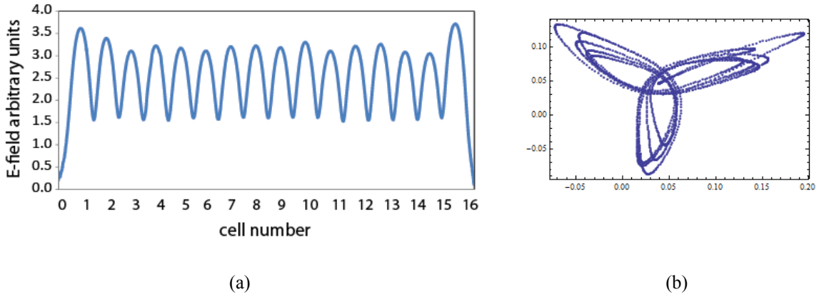
Figure 9: Field profile (a) and the Smith chart (b) measured with a bead pull in the tuned 16-cell PBG structure.
