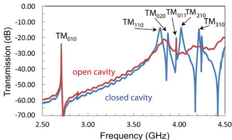
Figure 2. HOM measurement in the copper prototype with and with no outside copper enclosure.
