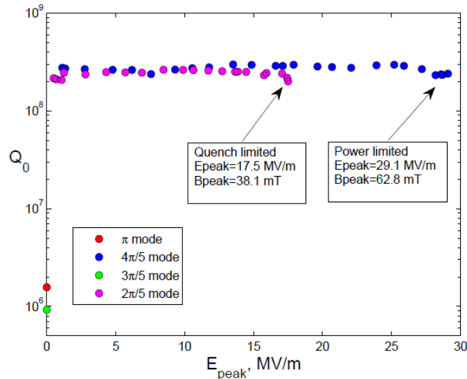
Figure 19: Q-factors for different modes in the 5-cell 2.1 GHz SRF cavity with the PBG cell as a function of the peak field on the surface of the cavity.
