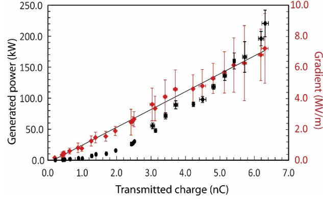
Figure 14: Power in the downstream coupling waveguide of the PBG structure as a function of the transmitted charge. The gradient in the structure computed from the measured power is also shown.
