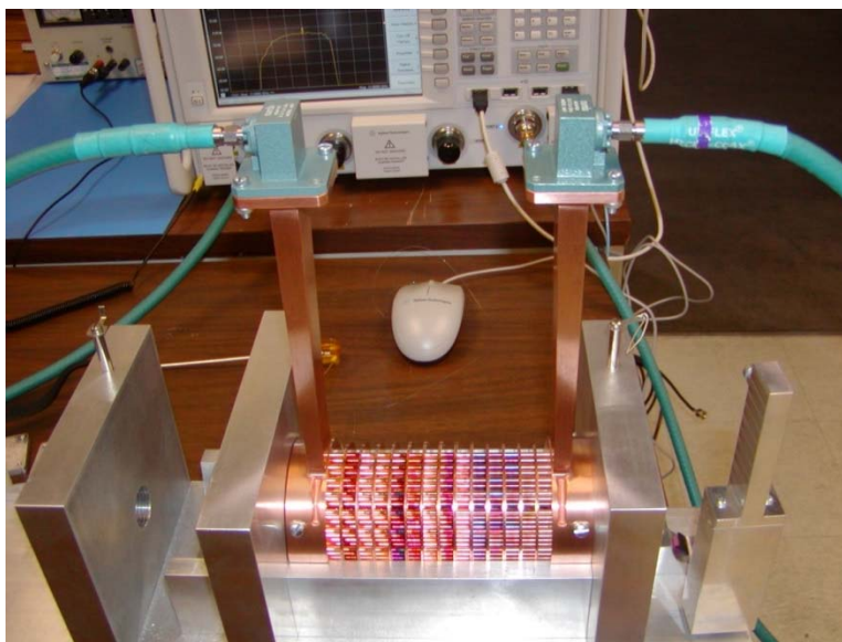
Figure 7: The 11.7 GHz PBG accelerating structure on a test bench.
