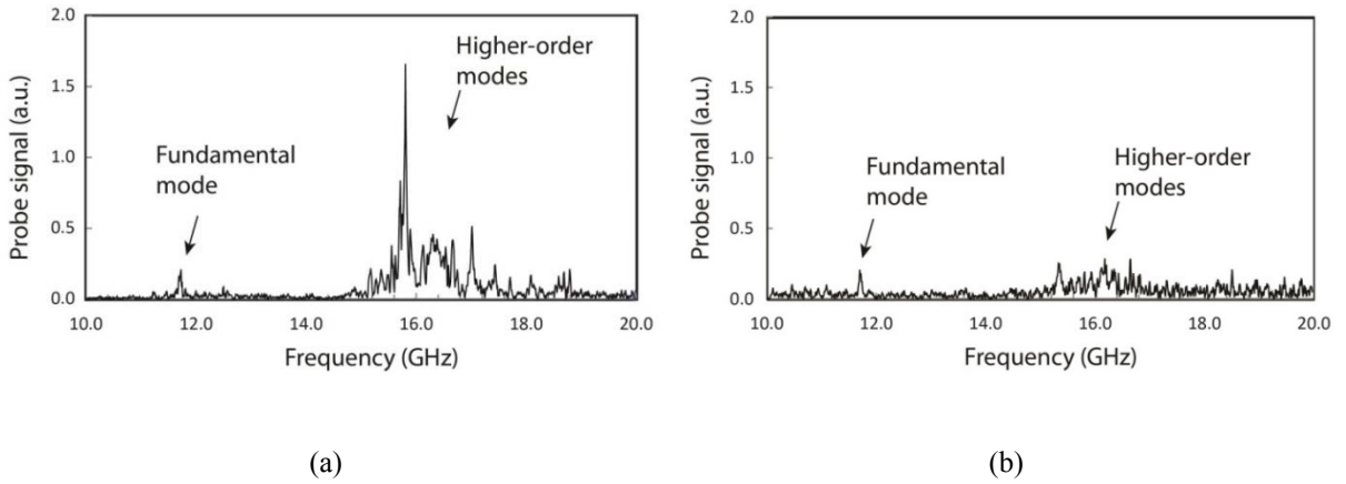
Figure 15: The rf spectrum of the signal picked up by a loop antenna at the periphery of the PBG structure: (a) the structure wrapped in foil; (b) the structure with 6 SiC absorbers.
