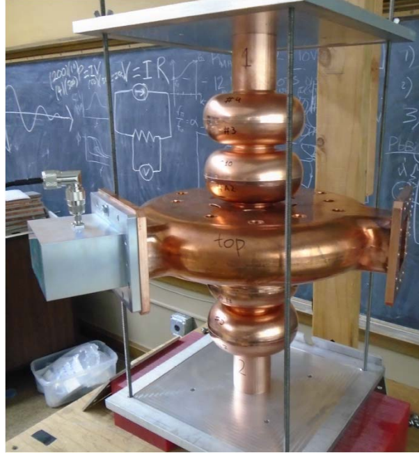
Figure 16: The copper prototype of the 2.1 GHz 5-cell SRF accelerating module with a PBG cell.
