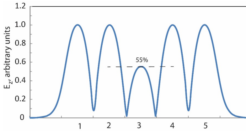
Figure 10: The profile of the electric field in the 2.1 GHz SRF accelerating module with a PBG coupling cavity.
