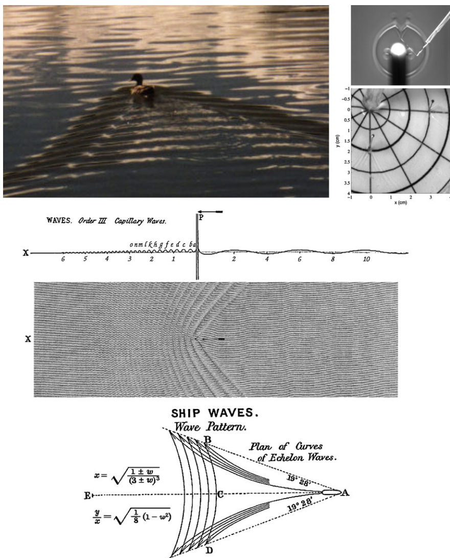
Fig. 6.6 Upper panels : picture of the Kelvin's ship-wave pattern behind a duck swimming at uniform speed on a quiet lake ( left ). Photograph courtesy of Fabrice Neyret, ARTIS-CNRS, France. Experimental picture of the Mach cone downstream of a wire immersed in radially flowing silicon oil ( upper right ). Capillary waves are not visible as they are quickly damped by the larger viscosity of silicon oil. Picture from [61]. Experimental picture of the Mach cone downstream of a pin immersed in very shallow flowing water: the surface wave dispersion is supersonic and the height modulation stays outside the Mach cone. Picture courtesy of Silke Weinfurter ( lower right ). Middle panel : Original hand drawing by John Scott Russell [62] of the waves generated by a vertical rod (diameter = 1/16 inch) moving along the water surface with a uniform velocity. The rod moves in the leftward direction: the capillary waves are visible in front of the rod and the gravity waves behind it. A cut of the surface height modulation is shown right above the main drawing. Lower panel : Original hand drawing by Lord Kelvin of Kelvin's ship-wave pattern [63]. The BCD wave-front belongs to the so-called transverse wave pattern. The so-called diverging waves connect the object at A to the dashed lines indicating the edges of the pattern
