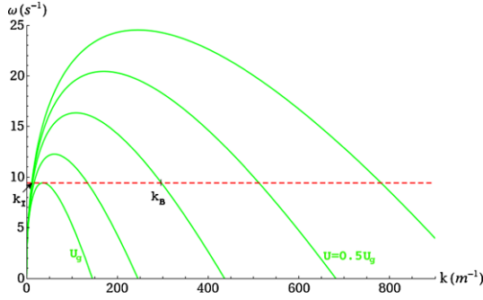
Fig. 7.9 Gravity waves and the trans-Planckian problem. For a given frequency \omega (dashed red line), a blue-shifted wave k_B is created from the incident wave k_I through mode conversion at the blocking line U = U_g . Since k_B has c_g < 0 , it moves away from the horizon towards lower |U| . As |U| \rightarrow 0 , k_B \rightarrow \infty , leading to a secondary trans-Planckian problem in flat spacetime
