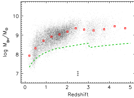
Fig. 16.6 Redshift distribution of the black hole masses of 14,434 QSOs selected from DSDR DR3, by Vestergaard et al. [49]. The median mass in each selected redshift bin is marked with a square. The median propagated black hole mass measurement error is shown in the midst of the lower part of the diagram . The dashed line refers to the faint SDSS flux limit so that at any given redshift observation can not pierce deep into the faint, lower mass end of the black hole mass distribution
