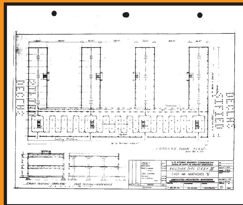
Design for Shop and Warehouse type B, by Associated Architects-Engineers, Los Alamos, New Mexico.
