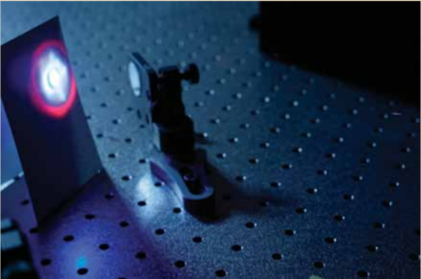
Figure 4 Bright white light generation from filamentation in air
