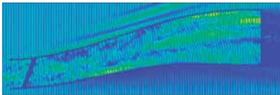
Figure 4 Total (scattered + incident) electric fields after computation using the DDM technique
