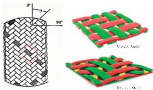
Figure 1 Fibrous braids in the form of Bi-axial or Tri-axial configurations
