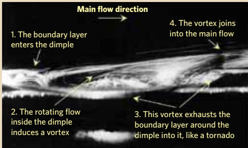
Figure 1 Illustration of TLJ vortex
