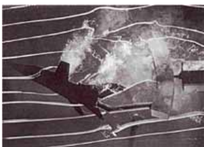
Figure 5 Flow separation of an aircraft at a high angle of attack
