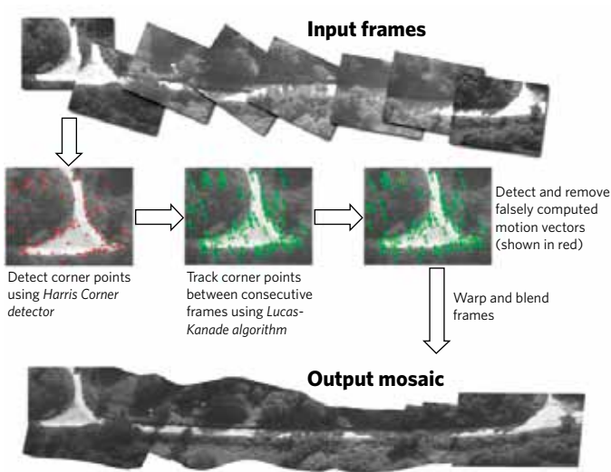
Figure 2 Video mosaicking algorithm
