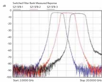
Figure 7 Measured performances of the SFB
