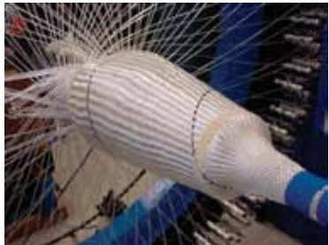
Braiding on mandrel
