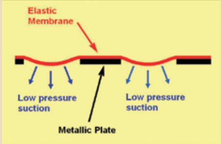
Figure 2 Dimple control concept used in TLJT airfoil study
