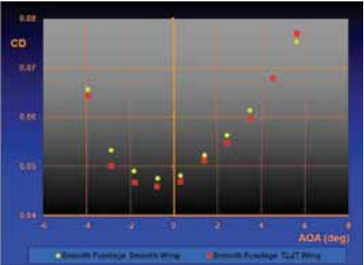
Figure 4 Comparison of drag measurement results of smooth and TLJT wings
