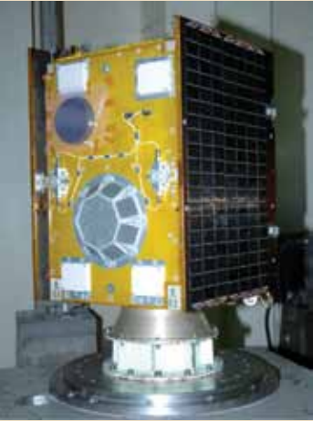
Figure 3 Centre of Gravity and Moment of Inertia measurements
