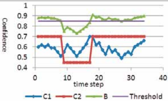
Figure 2 Combined confidence values vs. time step
