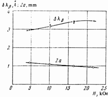
FIG. 7.3. Variation of the diameter of the discharge and line broadening as functions of the intensity of the magnetic field. Deuterium, p = 1.23 \text{ atm} , 9.7 \text{ kW} < 11.3 \text{ kW} .
