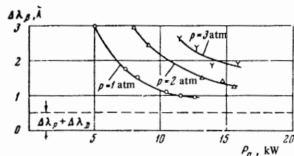
FIG. 3.2. The width of the D_\beta line as a function of the power input to the discharge in deuterium.
