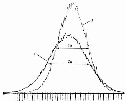
FIG. 2.3. A sample record of the intensity of emission of the D_\beta line for a filamentary discharge across a diameter. Deuterium, p = 1.4 atm. Curve 1— P_a = 8.0 kW, H = 1.6 kOe; curve 2— P_a = 8.7 kW, H = 21.7 kOe.
