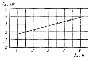
FIG. 5.2. Dependence of the current I_0 in the filament on the power input P_a determined from the experimental data for short filamentary discharges in deuterium. \circ — p = 1.37 atm, \times — p = 1.86 atm, P_a = 1.4 + 0.28 I_0 .
