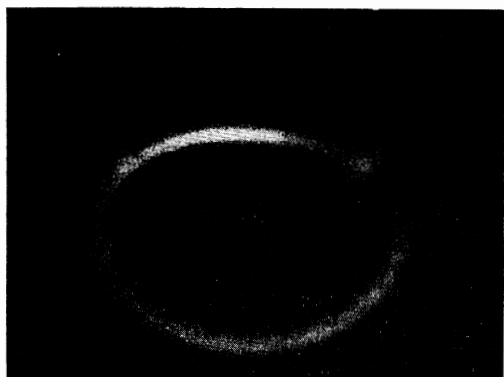
FIG. 1.4. Ring discharge in helium without stabilization by gas circulation. The reflection of the ring in the resonator wall can be seen. p = 1 atm, P_d = 1.8 kW, H_{01} (1960).
