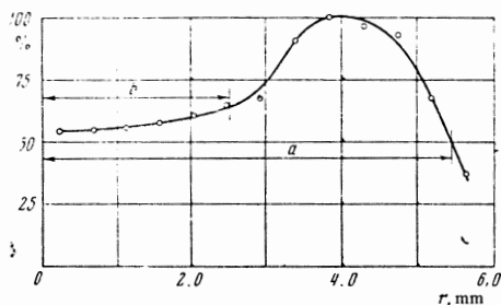
FIG. 3.7. Distribution of the volume intensity of emission ( \lambda \approx 5800 Å) along the radius of a high power discharge in deuterium calculated from the curve of Fig. 3.8. P_a = 14.3 kW, p = 1 atm.
