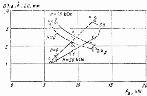
FIG. 7.1. Dependence of the diameter of the filament and of the broadening of the D_\beta line on the power in the discharge with a magnetic field and without it. Deuterium, 1.3 \text{ atm} < p < 1.5 \text{ atm} .
