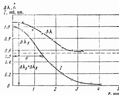
FIG. 3.3. Distribution of the Intensity I and of the width \Delta\lambda of the D_\beta line as a function of the radius of a discharge in deuterium. P_a = 6.5 kW, p = 1 atm.
