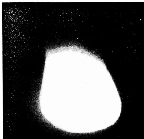
FIG. 1.3. Diffuse discharge with an admixture of acetone without stabilization by gas circulation. p = 200 mm Hg, P_a = 0.6 kW, H_{01} (1960).
