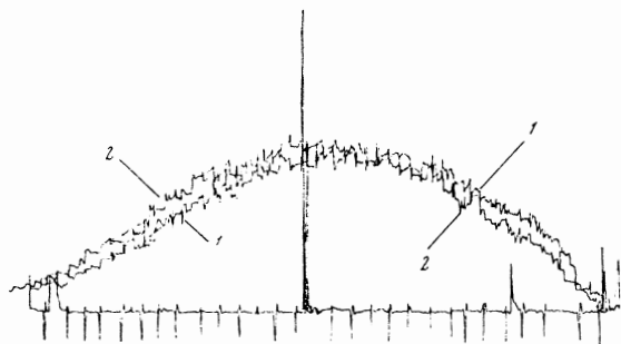
FIG. 4.3. Record of the distribution of intensities of the D_\beta (curve 1) and H_\beta (curve 2) lines along the diameter of the filament for the same mixture as in Fig. 4.2; P_a = 13 kW, p = 1 atm.
