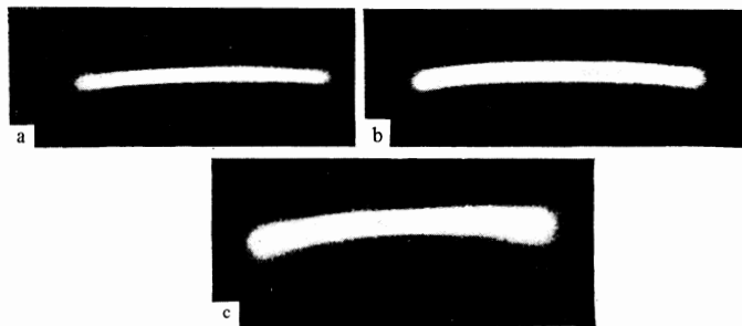
FIG. 1.2. Filamentary discharges in deuterium without stabilization by gas circulation, a— P_a = 2.9 kW; b— P_a = 4.5 kW; c— P_a = 6.4 kW, oscillations of H_{01} type (1961).
