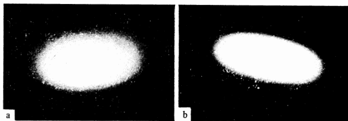
FIG. 1.1. Diffuse discharges in helium stabilized by gas circulation: a— p = 1.8 atm, P_a = 1.3 kW, b— p = 3.5 atm, P_a = 1.2 kW. Oscillations of E_{01} type (1963).
