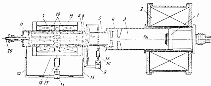
FIG. 2.1. Schematic diagram of the apparatus for the study of a filamentary discharge. 1—nigotron, 2—solenoid, 3—resonator, 4—spider transformer, 5—waveguide, 6—load resonator, 7—filamentary discharge, 8, 19, 20—windows, 9, 13—centrifugal air blowers, 10, 17—heat exchanger, 11—piston, 12—legs of the "spider," 14, 15—tubes, 16—a number of apertures for the passage of gas, 18—solenoid.
