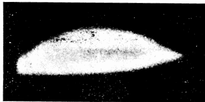
FIG. 3.6. Photograph of a filamentary discharge in deuterium with an admixture of 5% argon at high power P_a = 14.7 kW and high pressure p = 3.32 atm. Length of the discharge \sim 10 cm. The left edge of the discharge is blocked by the window. Oscillations of E_{01} type (1969).
