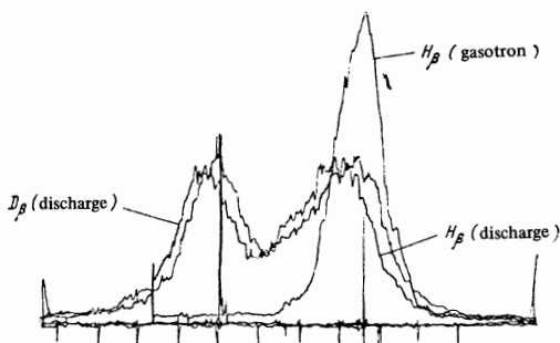
FIG. 4.2. Record of the D_\beta and H_\beta lines in a mixture of 50% D and 50% H. P_a = 13 kW, p = 1 atm. The spectrum of the discharge has been recorded twice.
