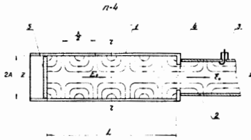
FIG. 5.1. Structure of the HF field in a resonator for E_{01} oscillations.
