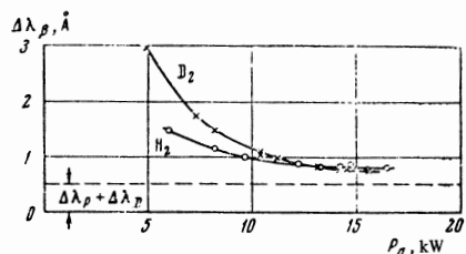
FIG. 3.4. Widths of the D_\beta and H_\beta lines as a function of the power input to the discharge.
