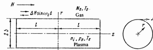
FIG. 8.2. Notation adopted for making calculations concerning radial magnetoacoustic waves in the plasma of the filament.
