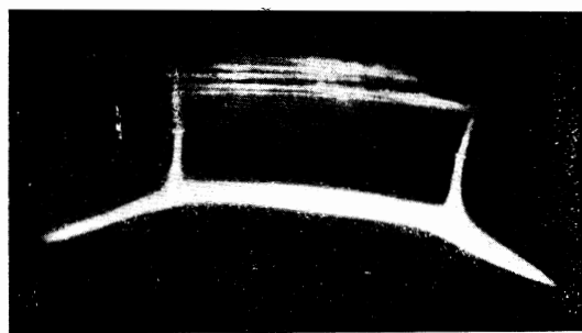
FIG. 1.5. Filamentary discharge in deuterium whose legs have stuck to the resonator wall where its reflection can be seen. p = 1.8 atm, H_{01} (1961).
