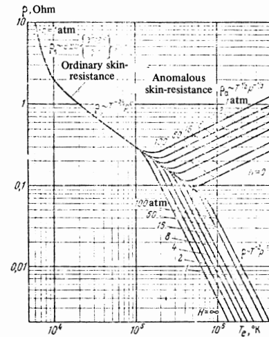
FIG. 6.1. Total skin-resistance as a function of the temperature of the electrons in the plasma calculated for a frequency \omega = 10^{10} .
