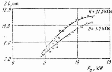
FIG. 7.2. Dependence of the length of the filamentary discharge on power input at low and high magnetic fields. Deuterium, 1.3 \text{ atm} < p < 1.46 \text{ atm} .
