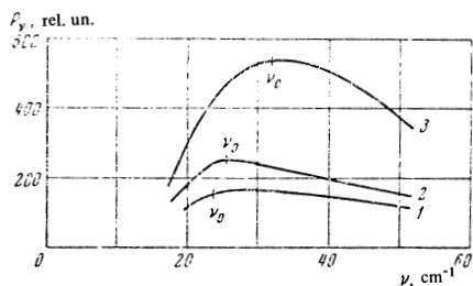
FIG. 3.5. Intensity of emission from a filamentary discharge in deuterium in the far infrared region of the spectrum. Curve 1— p = 1 atm, P_a = 8.8 kW; curve 2— p = 1 atm, P_a = 12 kW; curve 3— p = 2 atm, P_a = 14.7 kW.
