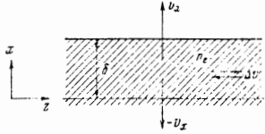
FIG. 6.2. Schematic diagram for calculation of the anomalous skin-resistance.
