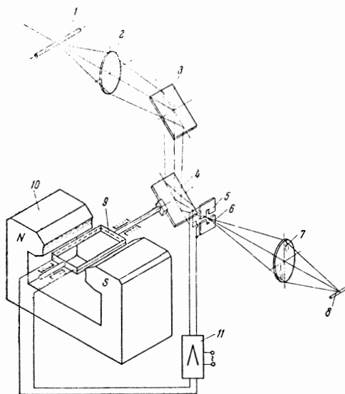
FIG. 2.2. Schematic diagram showing the principle of the stabilizer of the image of the discharge on the slit of the spectrograph. 1—discharge, 2, 7—lenses, 3, 4—mirrors, 5, 6—photoresistors, 8—image of the filament, 9—frame, 10—magnet, 11—control unit.
