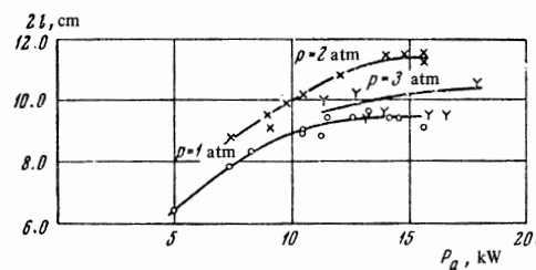
FIG. 2.5. Variation in the length of a filamentary discharge in deuterium as a function of the power input.
