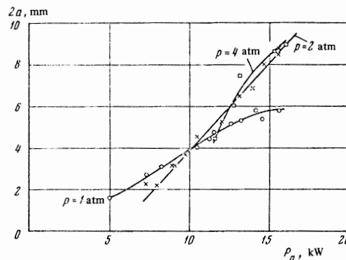
FIG. 2.4. Curves of the dependence of the diameter of a filamentary discharge in deuterium on the power input.
