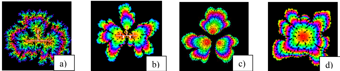
Fig.9. DLA with a variation in the statistics of the deposited particle diffusion. Simulation with the Hurst exponent of diffusion: (a) H=0.5 , (b,c,d) H=0.8 .
