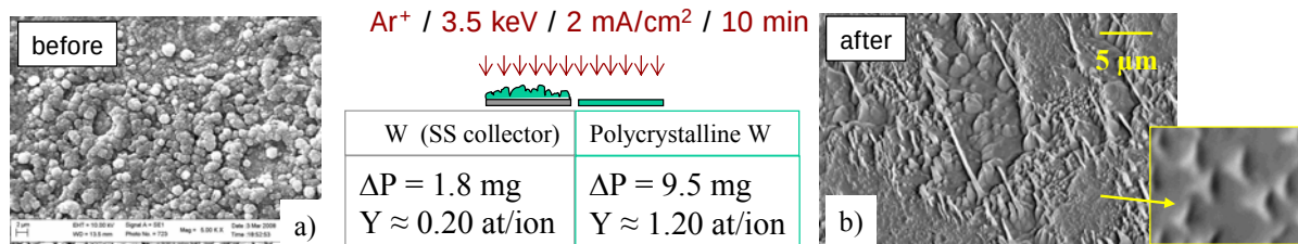
Fig.5. \text{Ar}^+ sputtering of W dusty film. a) before modification (b) after modification
