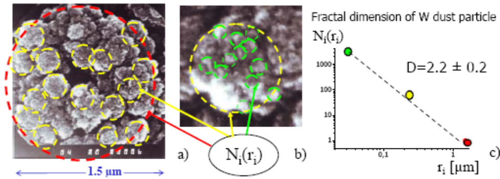
Fig.8. QSPA dust hierarchical structure (a,b) and fractal dimension (c).
