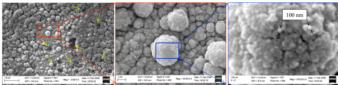
Fig.2. QSPA. Dust particles after W target erosion with 1.5 MJ/m 2 energy load.
