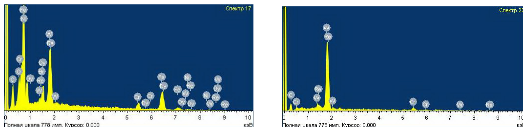
Fig.4. Auger spectrum of W dust. a) on the surface, b) in deeper layer
