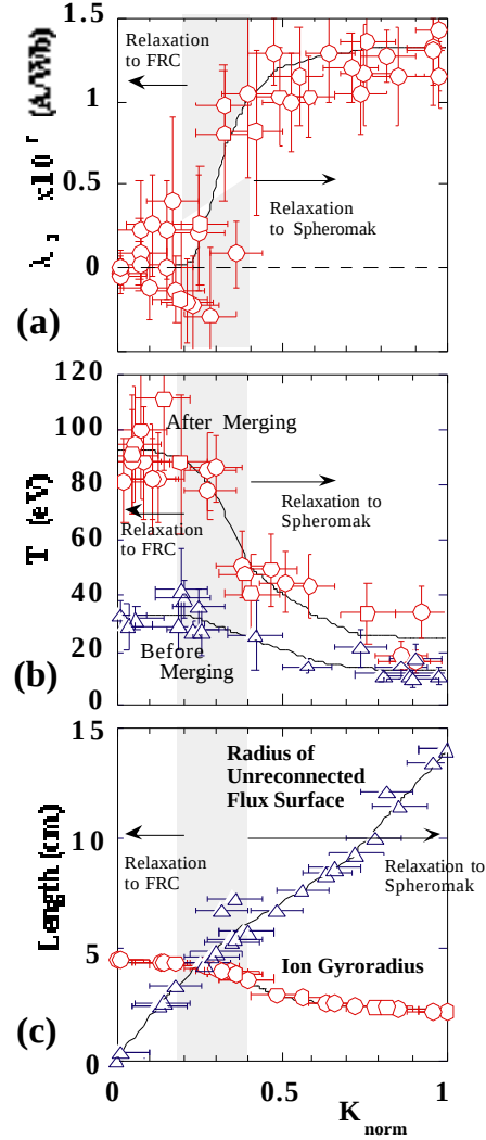
FIG. 3 Dependence of poloidal eugenvalue (a), ion temperature (b), ion gyroradius and radius of unreconnected flux surface (c) as a function of initial helicity K_{norm} normalized by the value for the Taylor state.
