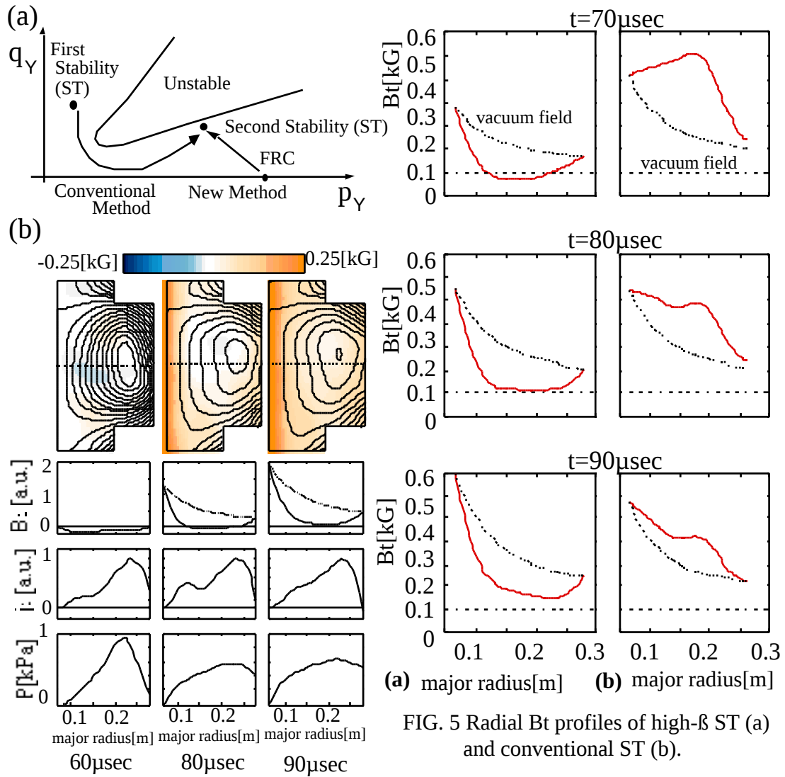
FIG. 4 Basic idea of forming high- \beta ST in s-a diagram (a), r-z contours of poloidal flux and toroidal field strength and radial profiles of B_t , j_t and thermal pressure p of the FRC and the produced high- \beta ST (b).
