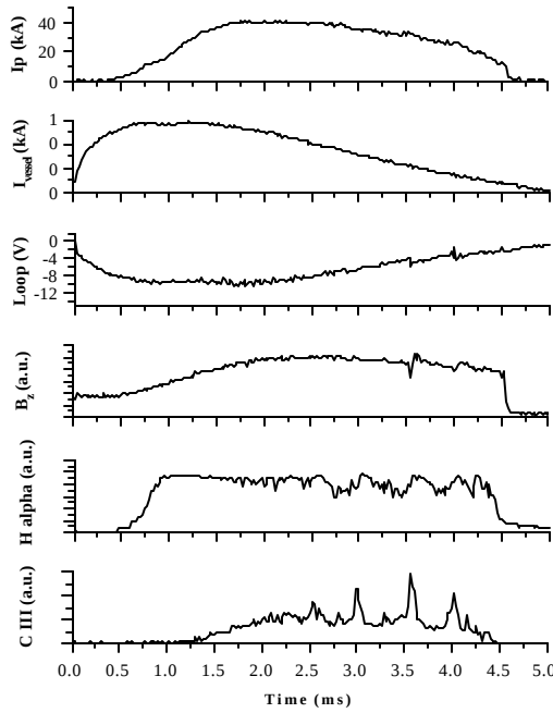
Figure 5: Electromagnetic and optical signals from ETE discharge: plasma current ( I_p ), induced vessel current ( I_{vesse} ), loop voltage (Loop), vertical magnetic field ( B_z ), H-alpha emission (H alpha) and carbon three emission (CIII).
