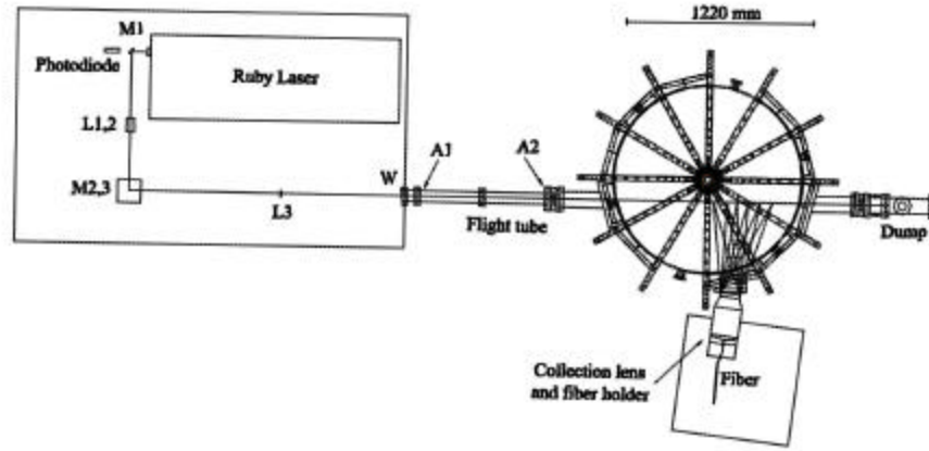
Figure 3: Top view of the ETE Thomson scattering system. M1,2,3 are mirrors; L1,2 are beam expander lenses; W is the beam injection window and A1,2 are apertures.
