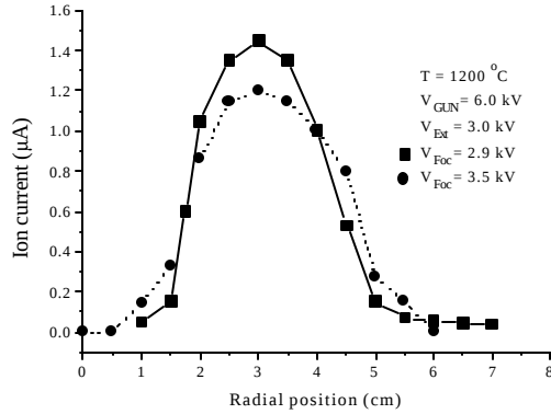
Figure 8: Radial beam profiles of the FNLB at the neutralizer for two different geometry of the ion gun. The temperature of the ion source was 1200^{\circ}\text{C} and the best voltage values for each configuration are shown ( V_{\text{GUN}} – acceleration, V_{\text{Ext}} – extraction, V_{\text{Foc}} – collimation).
