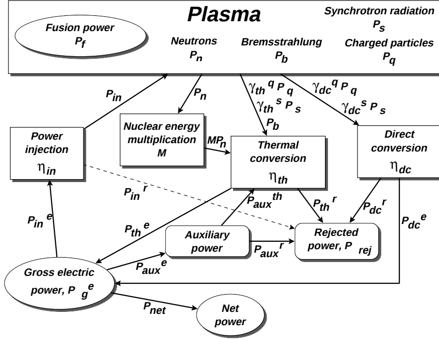
Figure 3: FRC plasma and plant power flow.
