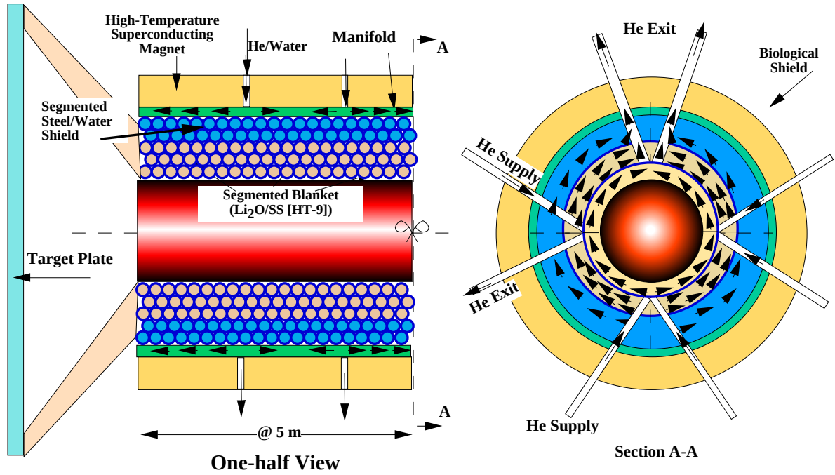
Figure 1: One-half view and cross section of a preliminary concept for the tritium-breeding blanket.
