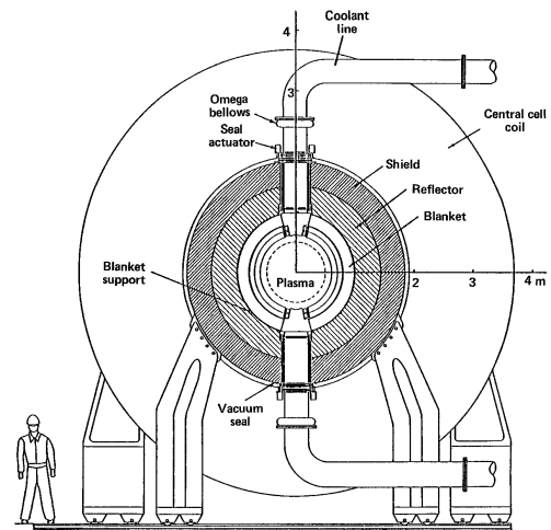
Figure 2: Cross section of the MARS tritium-breeding blanket.
