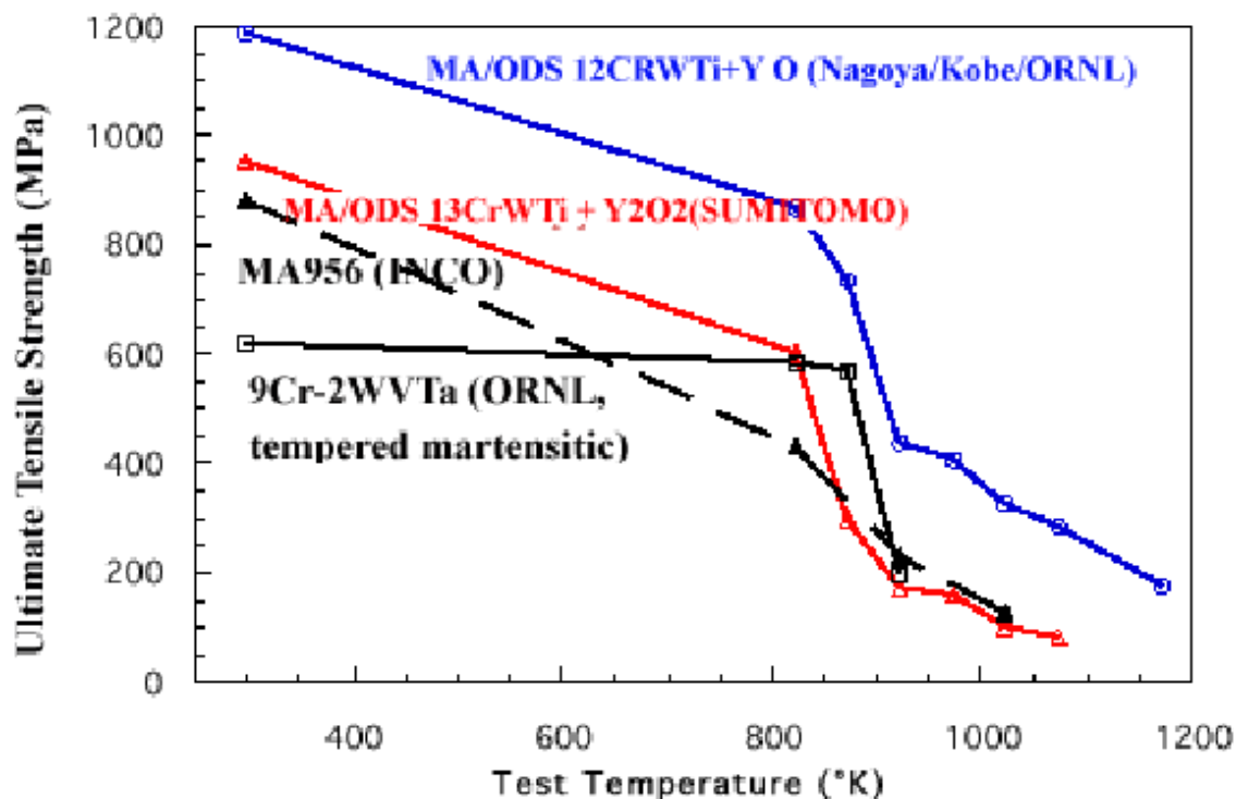
Figure 2-1: Comparison of the temperature-dependent tensile strengths of oxide dispersion strengthened and ferritic-martensitic (9Cr-2VTaW) steels.
