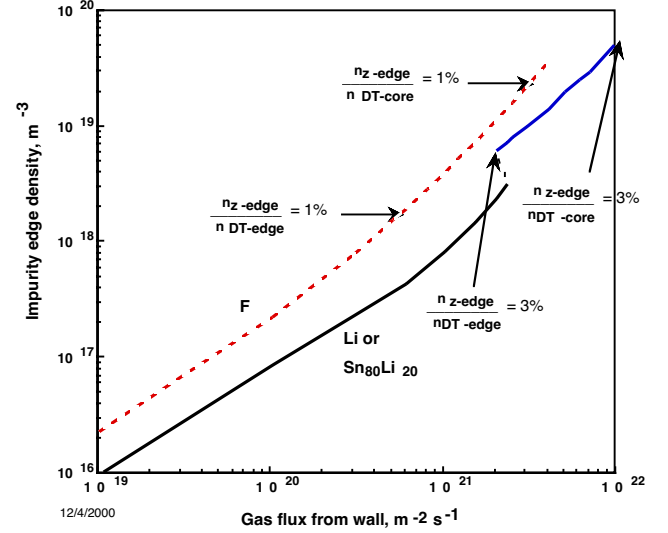
Fig. 10. Plot of impurity edge density vs average evaporation rate.
