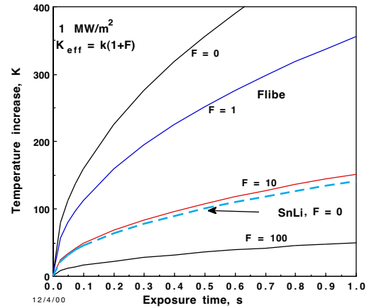
Fig. 6. Temperature rise of the fluid element versus time at 1.0 MW/m 2 . F is the thermal conductivity enhancement factor to account for near surface turbulence or convection.
