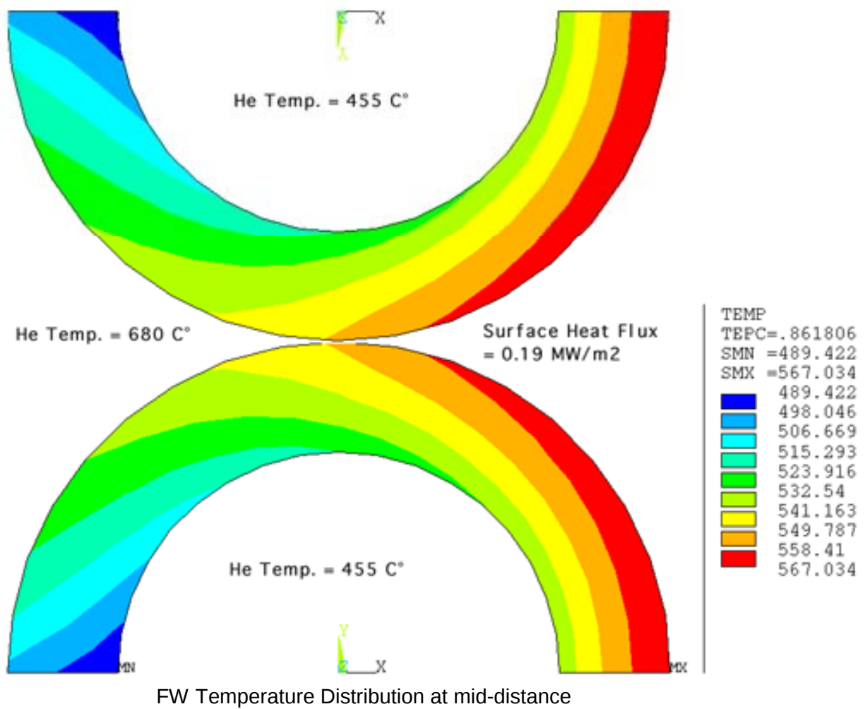
Figure 2-12: Temperature distribution at the mid-point of the inlet and the outlet of the first wall.
