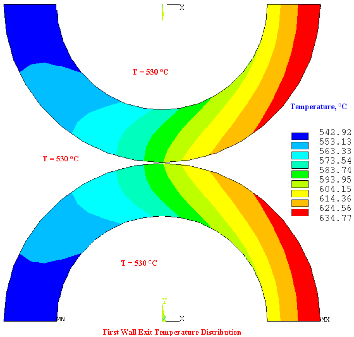
Figure 2-13: Temperature distribution at the exit of the first wall.
