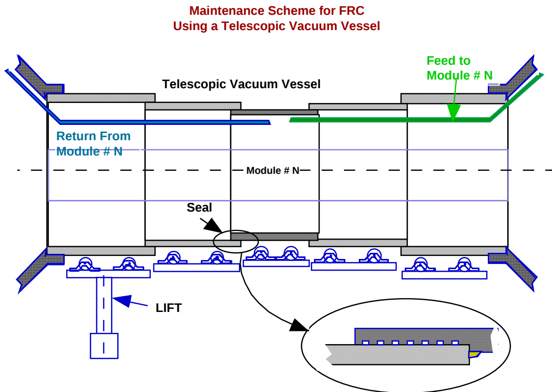
Figure 2-15: Maintenance scheme for D-T FRC Scoping Study Fusion Core.
