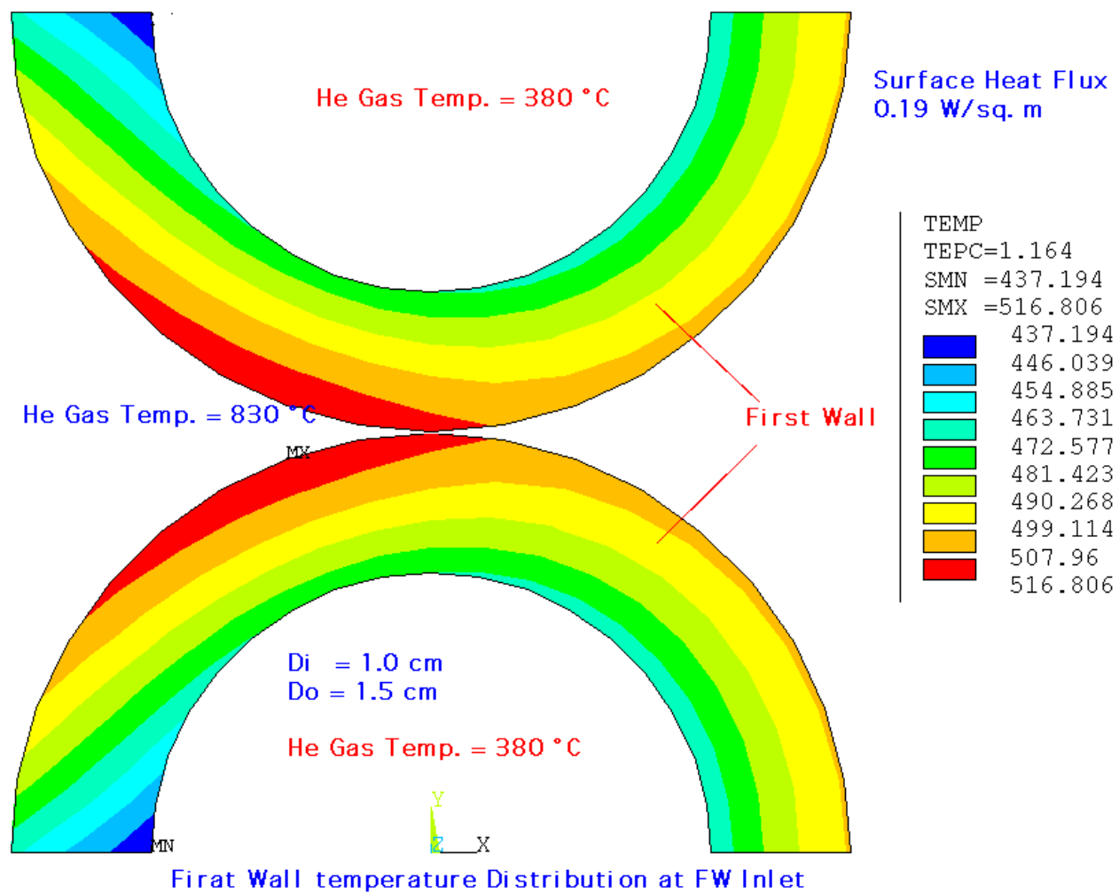
Figure 2-11: Temperature distribution at the inlet of the first wall.
