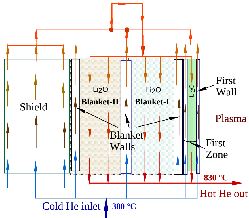
Figure 2-6: Coolant routing in the FRC first wall blanket and shield.
