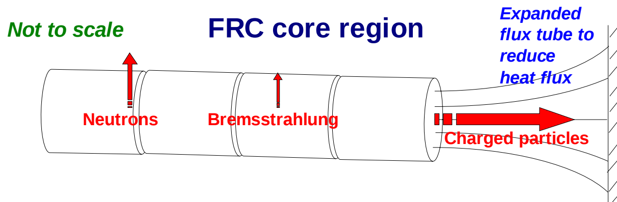
Figure 1-1: Energy flow from the FRC fusion core.
