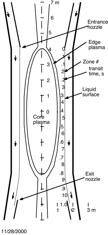
Figure 8. The FRC liquid flow model is shown. The flow path is in on one end and out on the other about 10 m in length.
