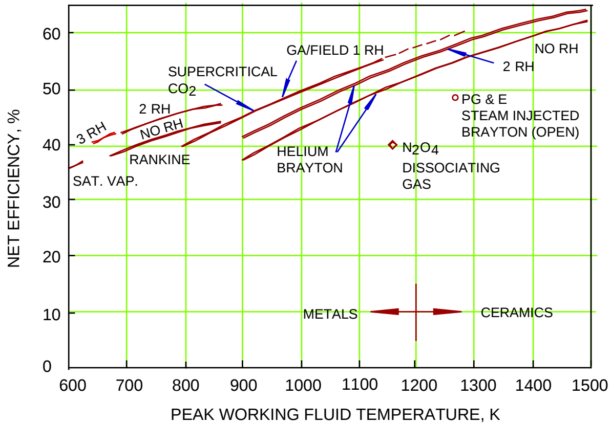
Figure 2-7: Net efficiencies vs. peak temperature for several power cycles: steam, Brayton, and GA/Field cycles (extracted from Ref. 3).
