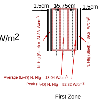
Figure 2-2: A sketch of the radial build of the FRC and nuclear heating in each zone.
