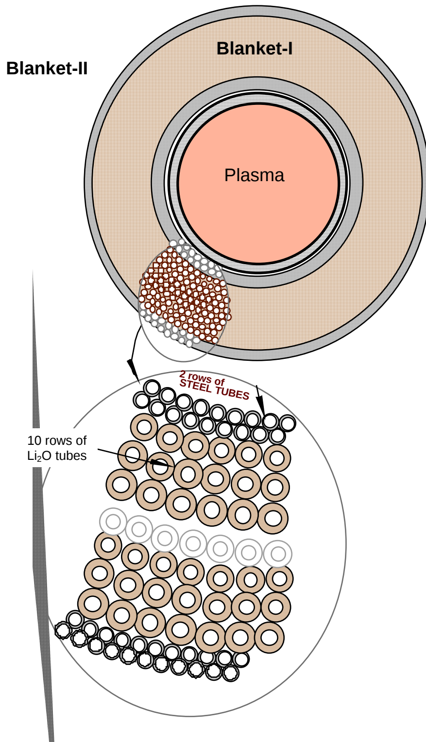
Figure 2-5: Detailed cross section of blanket-I with the plasma in the core of the FRC.
