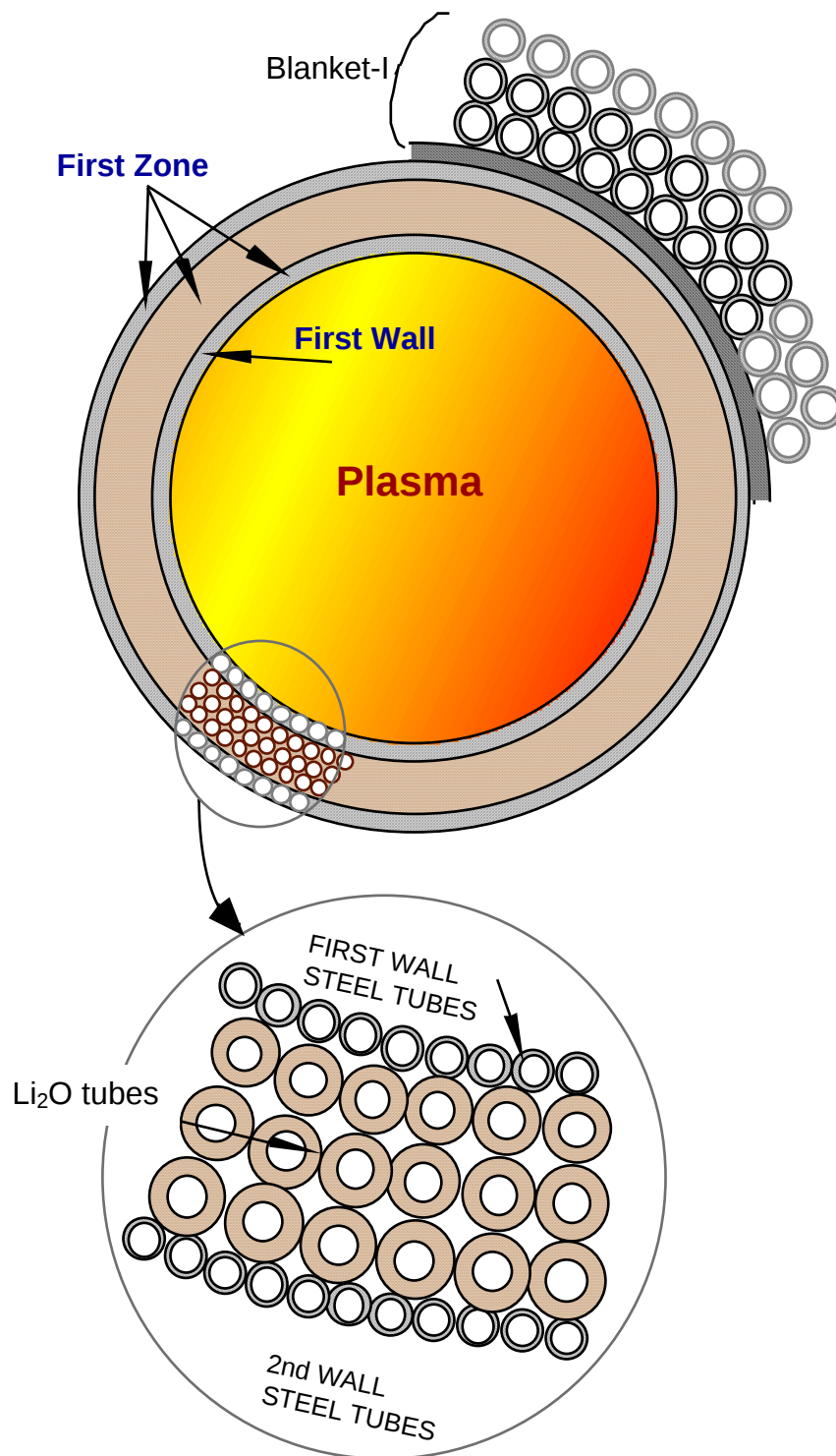
Figure 2-4: Detail of the first zone of the FRC.
