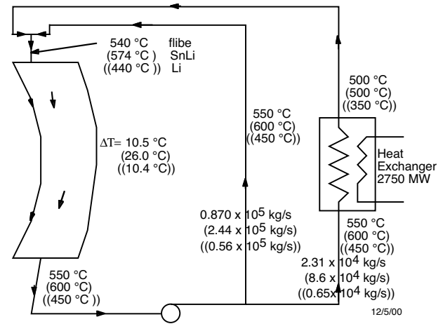
Fig. 4. Mass flow and temperature diagram for the FRC. The numbers shown are for flibe with the SnLi values shown in parentheses and Li, 1 m thick, in double parentheses
