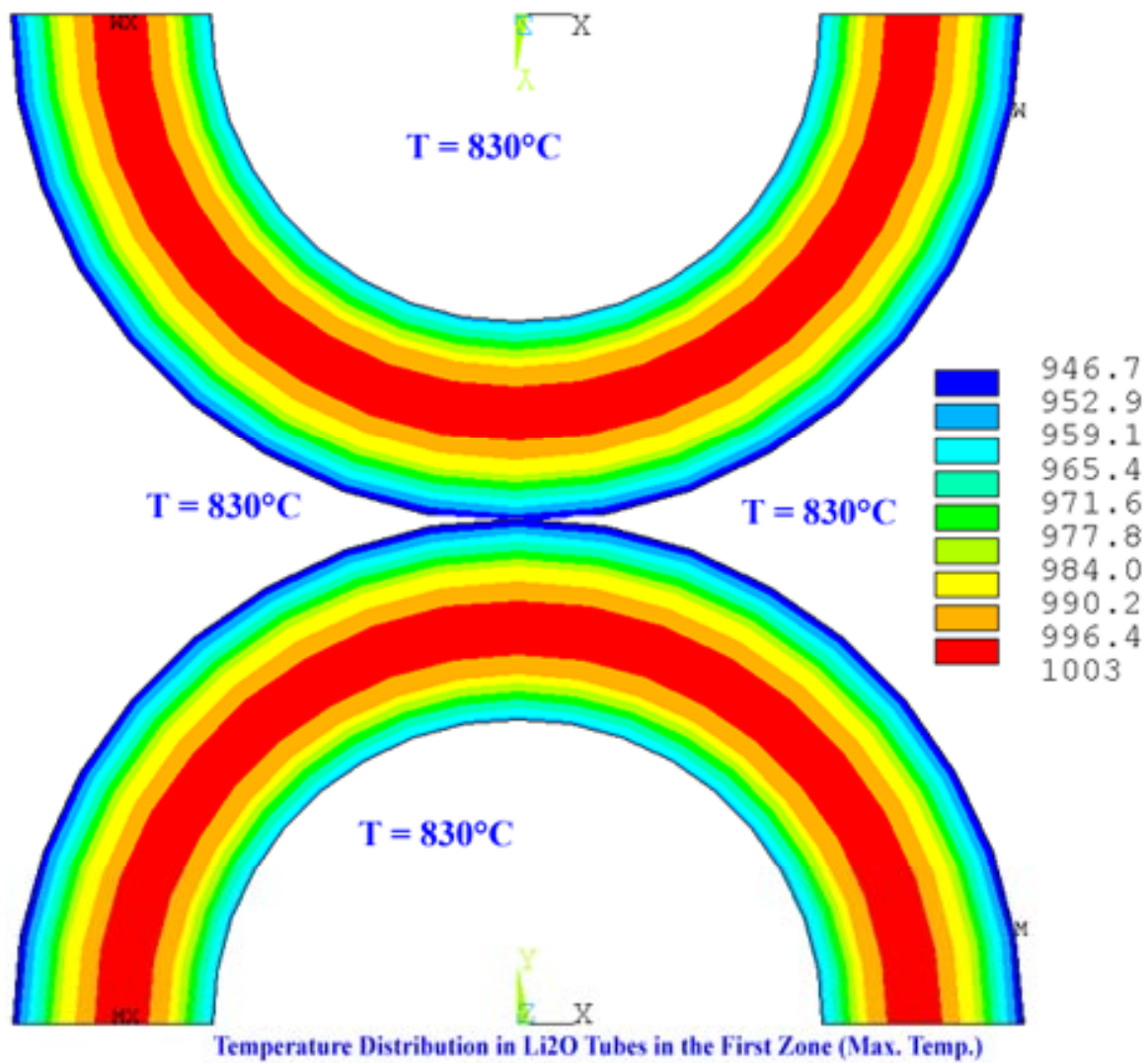
Figure 2-14: Temperature distribution at the exit of the first zone Li 2 O tube.
