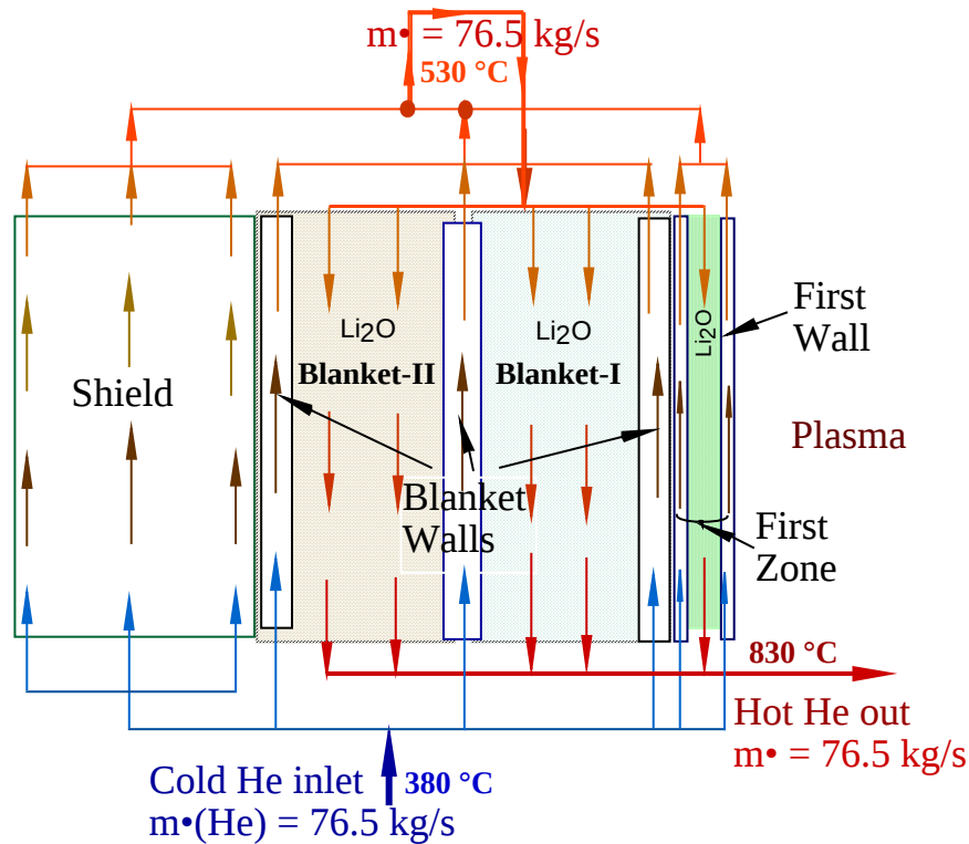
Figure 2-8: Helium coolant routing and the corresponding helium coolant mass flow rate and temperature at inlet and exit of FRC components.
