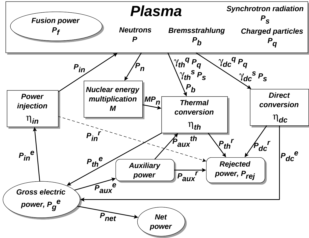
Figure 3-1: Plasma power flow for an FRC fusion power plant.
