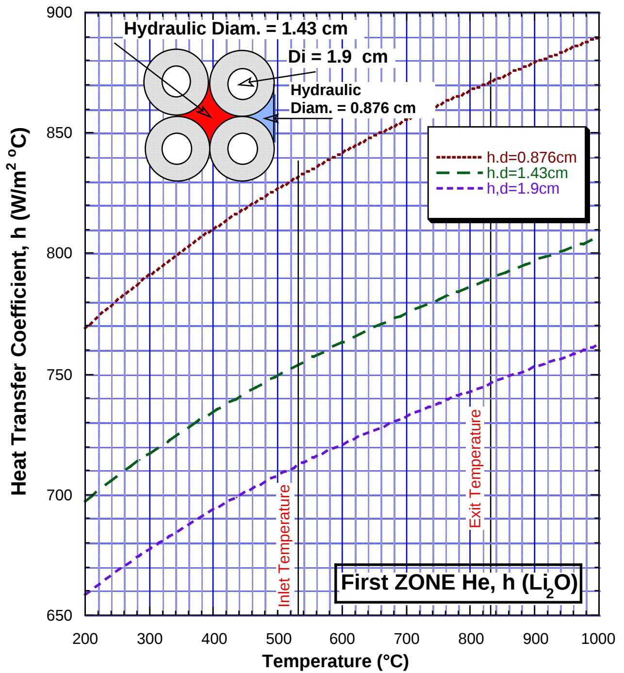
Figure 2-10: Heat transfer coefficient of coolant helium in the first zone Li_2O tubes.
