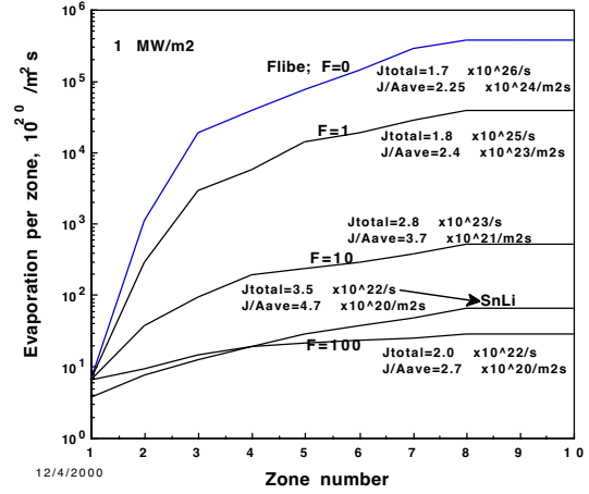
Figure 9. Evaporation per zone and total evaporation for FRC for 1 MW/m 2 .
