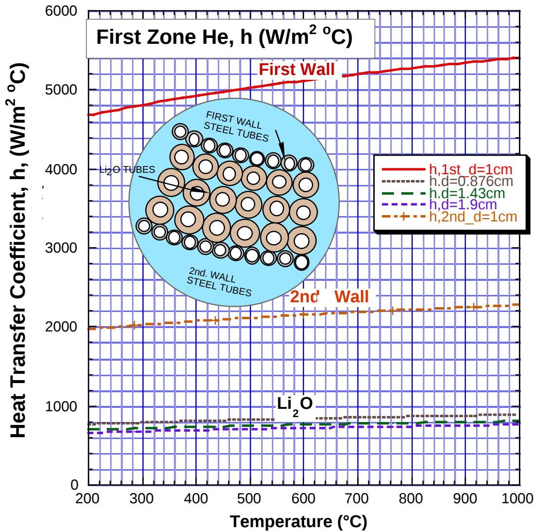
Figure 2-9: Heat transfer coefficient of coolant helium in the first zone (First wall, first zone \text{Li}_2\text{O} tubes, and second wall).
