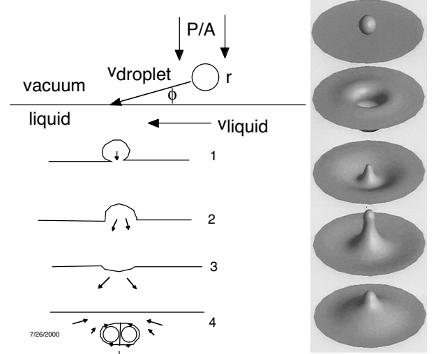
Fig. 5. The idea of droplets sprayed on a surface causing convection with no splash is shown on the left. A simulation is shown on the right with Reynolds number = 2vr/v = 20 and Weber number = \rho r v^2 / \sigma = 2 .
