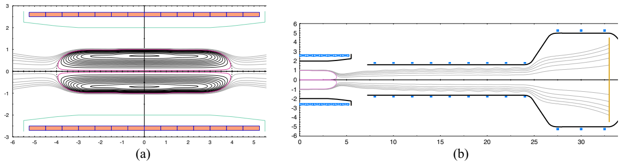
Figure 2. FRC configuration. The magnetic flux surfaces from an MHD equilibrium calculation using the Corsica code are shown in (a) and the flux surfaces leading out to the end tanks are shown in (b).
