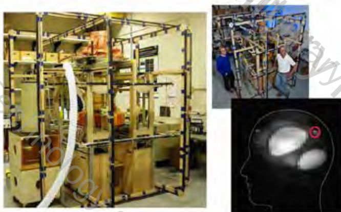
Figure 4. The unshielded SQUID-based detection system that allows performing both ULF MRI and SPMR signals detection in urban locations. The right bottom image shows ULF MR Image recorded using a phantom of the human brain with a small (1 cm) inclusion.
