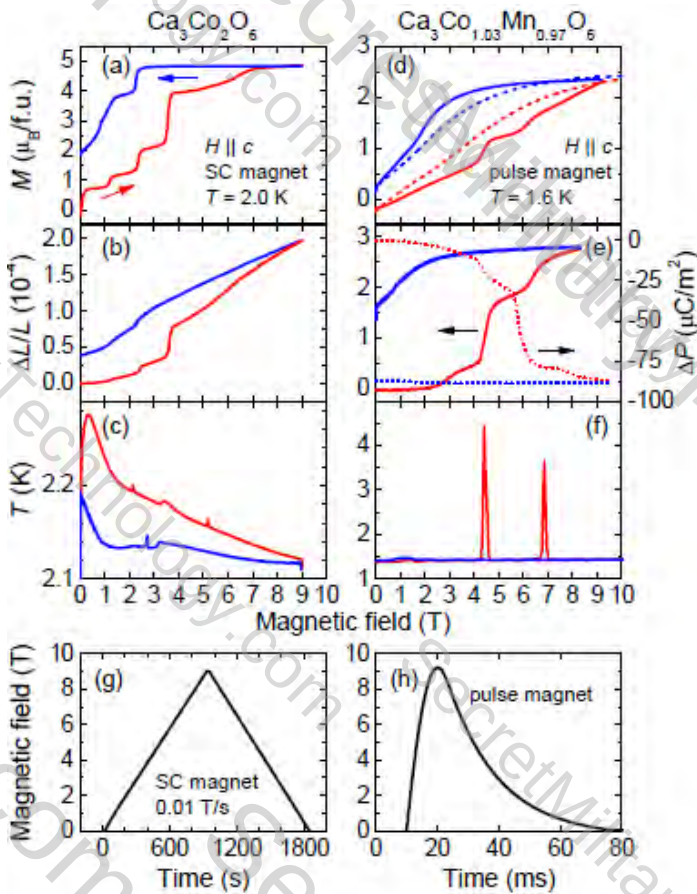
Figure 2. Steps in the magnetization M , relative length change DL/L , magnetocaloric effect (change in temperature T with magnetic field H ) and electric polarization P of \text{CaCoO} and \text{CaCoMnO} , verified in multiple samples. The steps occur for sweep rates dH/dt above 1.6 \times 10 \text{ T/s} for \text{CaCoO} , and between 74 and 1,400 \text{T/s} for \text{CaCoMnO} . (g) and (h) show the magnetic field vs time profile for the SC (superconducting) and pulsed magnets used in this study. [10]
