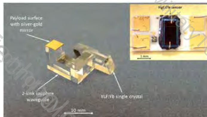
Figure 4. Picture of assembly consisting of a high-purity yttrium-doped yttrium-lithium-fluoride (YLF:Yb) crystal and a two-kink sapphire waveguide. The YLF:Yb crystal input and output faces were cut at Brewster's angle in order to minimize reflection losses for the pump laser. The sapphire crystal was attached to the YLF:Yb crystal by a diffusion-bonding process that eliminated the use of adhesives, which could introduce parasitic heating. The two-kink sapphire waveguide provided a good thermal link between the crystal and the payload while preventing light from the crystal to reach the payload. A silver-gold mirror was deposited at the end of the sapphire waveguide for additional light rejection. The mercury-cadmium-telluride (MCT) infrared sensor (pictured in the inset) was mounted on top of the gold mirror.
