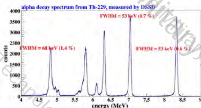
Figure 4. Double-sided silicon strip detector was calibrated for channel-to-energy and an energy resolution. Pulse height histogram was measured with a Th-229 radioactive source.
