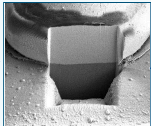
High-magnification scanning electron microscopy image of a focused ion beam cross-section from a bond-wire area in an unaged diode.
