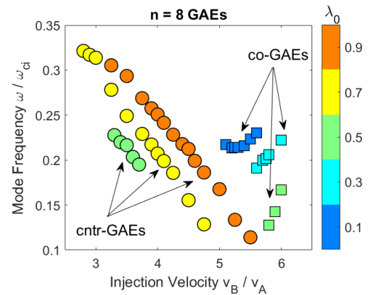
Fig. 3 Change in frequency for |n|=8 GAEs as a function of the normalized beam injection velocity. Cntr-GAEs are marked by circles, co-GAEs by squares. Color denotes the central pitch \lambda_0 = \mu B_0 / \epsilon of the beam distribution in each simulation. On-axis cyclotron frequency is 2.4 MHz. Reproduced from Phys. Plasmas 25 (2018) 042508, with the permission of AIP Publishing.
