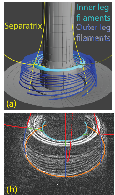
Figure 8: (a) Rendering of the NSTX-U divertor with flux tubes corresponding to divertor-localized fluctuations; (b) Divertor image in C III emission (9 \mu s exposure) after high pass filtering. Separatrix (red), inner (green) and outer (blue) divertor legs, inner (cyan) and outer (orange) strike points are overlaid.
