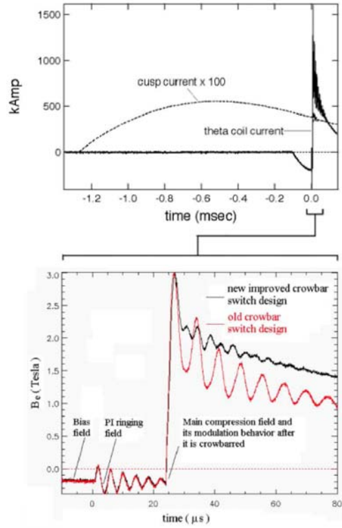
Figure 1: (upper) Long time scale current in the \Theta and cusp/mirror coils. The cusp current creates a B_z opposite to the initial bias B-field. In this case the main bank fires at t = 25 \mu s and rings while the crowbar forces the current to monotonically decay with its L/R time. (lower) Waveforms from one of the magnetic probes (located on the top of \Theta -coil segment B) recorded during a shot with the old crowbar switch (red) and with the new crowbar switch (black).
