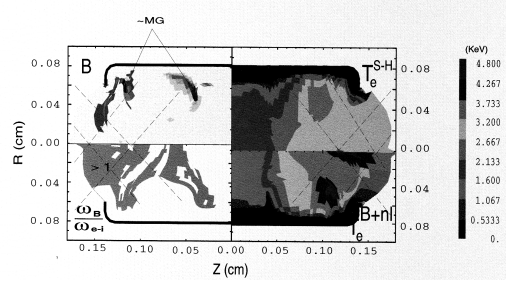
Fig. 4 : Electron temperature maps calculated with Spitzer-Härm (S-H) or new model (B+nl), at maximum laser power time. Localization of B-fields is shown, with level.
