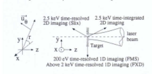
Fig. 1 : Experimental set-up
