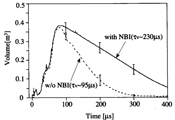
Fig. 5 Time evolution of separatrix volume in the case of mirror ratio R_M = 8 . The characteristic decay time \tau_v of the volume increase from 95 \mu s to 230 \mu s with NB injection.
