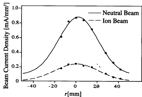
Fig. 3 Radial distribution of the beam current density at z = 600 \text{ mm} in case of 5 kV of accelerating voltage and 3.0 A of current.
