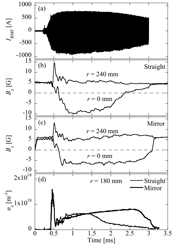
Fig. 4. Time evolutions of (a) RMF current I_{\text{RMF}} , (b) B_z in straight configuration, (c) B_z in mirror configuration, and (d) electron density n_e .
