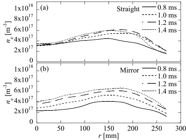
Fig. 8. Radial profiles of n_e in (a) straight and (b) mirror configurations of bias magnetic field.
