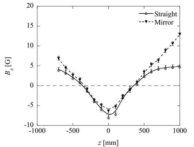
Fig. 7. Axial profiles of B_z at t = 1.4 ms in straight and mirror configurations.
