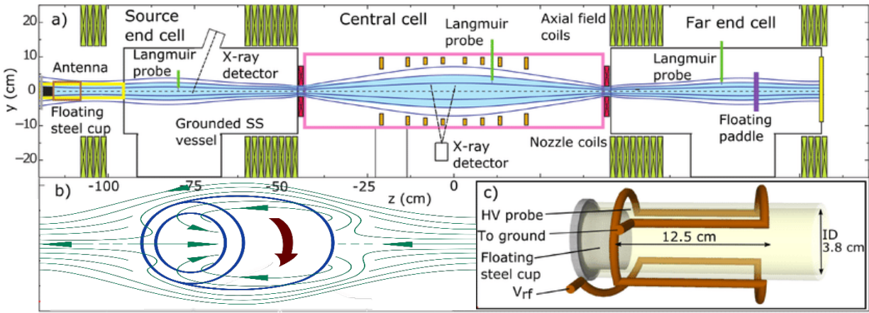
Figure 1: Simplified Schematic of the PFRC-2
