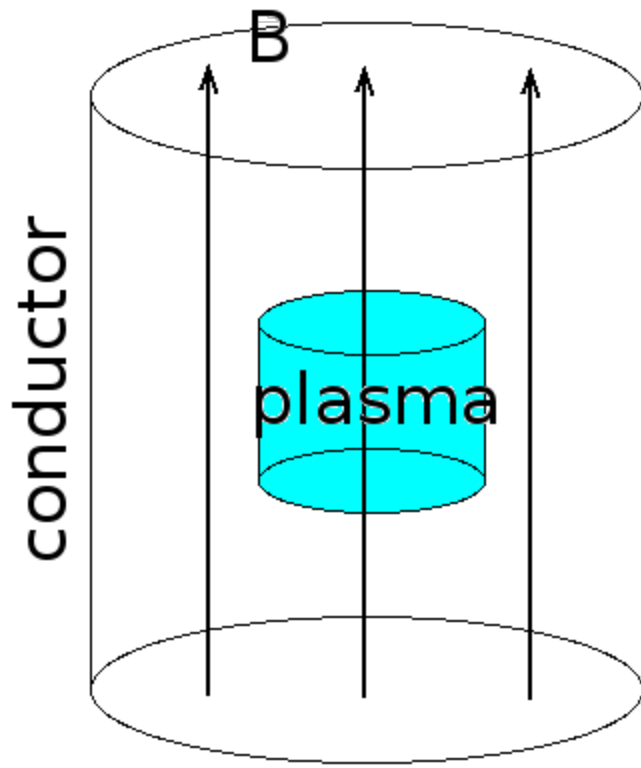
Figure 2: Case where a plasma inside a conducting cavity expands with a background magnetic field producing diamagnetic currents.
