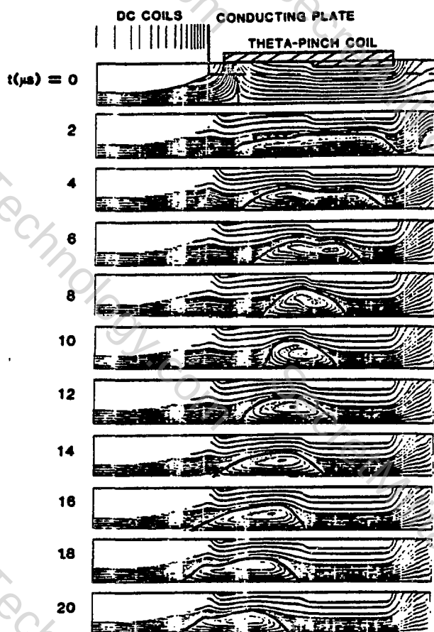
Fig. 1. Simulation of FRC formation and translation initiation with a conducting plate separating the DC coils and theta-pinch coil. Flux contours are shown with the separatrix indicated by a bold line.
