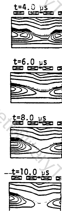
Figure 4. Two-cell formation. Filling pressure 7 mTorr.
