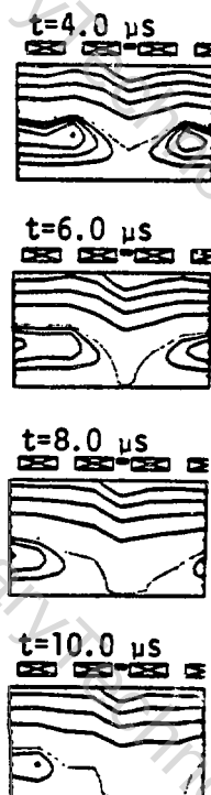
Figure 3. Two-cell formation. Filling pressure 5 mTorr.
