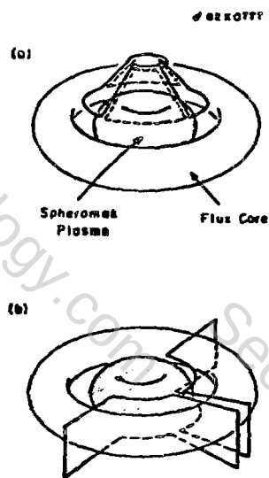
Configuration of figure-8 and saddle coils Figure 2
