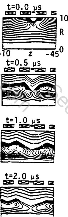
Figure 4. Two-cell formation. Filling pressure 7 mTorr.
