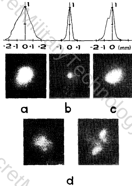
FIG. 3. X-ray photograph of electron focal spot and distribution of its intensity. a – time-integrated curve, b – 45 ns after current start, c – 70 ns after current start, d – current channel destruction on several separate filaments.
