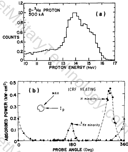
FIG.3. Energetic particle measurements. (a) Proton spectrum from D-^3\text{He} reactions and (b) bolometer probe measurements for P_{\text{RF}} \approx 1 \text{ MW} (for H minority case, the OH level has been subtracted).
