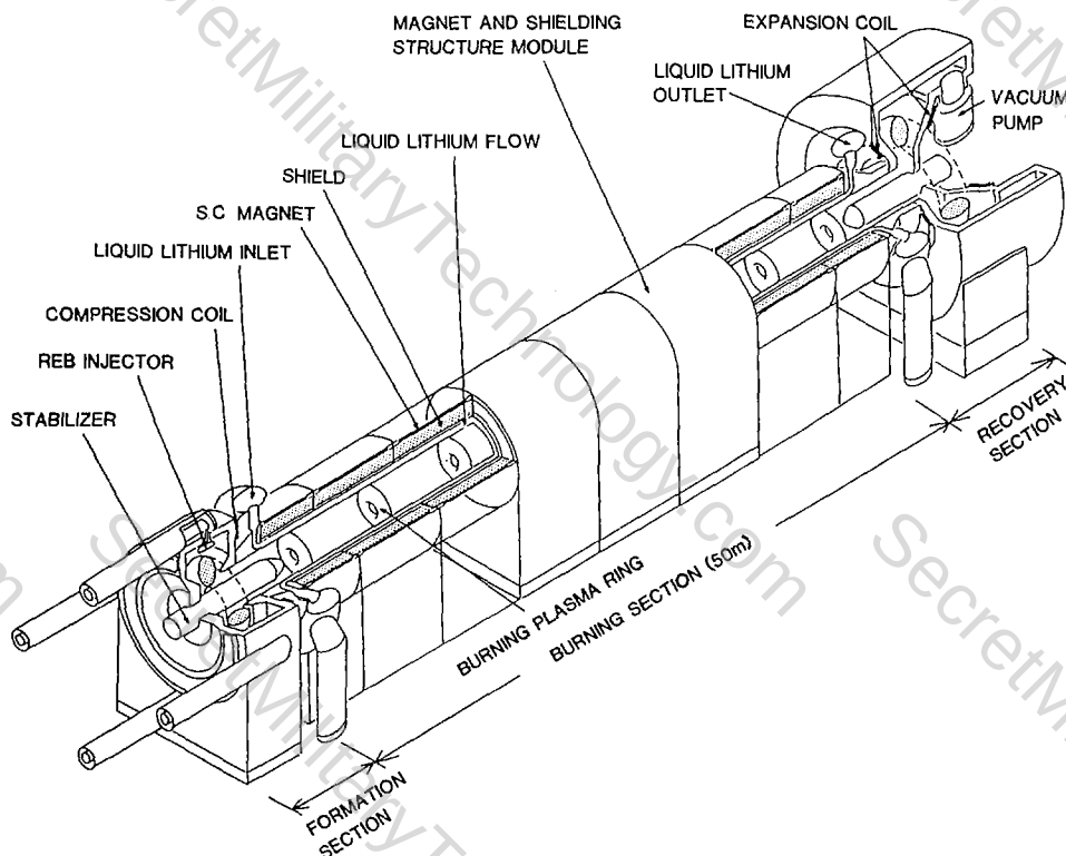
FIG.1. Layout of the moving-ring reactor system KARIN-I.
