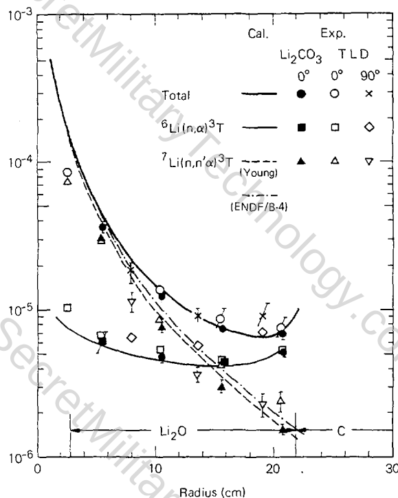
FIG.4. Tritium production rate distribution in \text{Li}_2\text{O}-\text{C} assembly.
