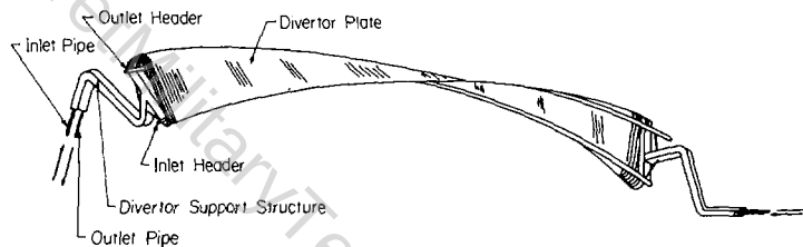
FIG.11. View of divertor plate.
