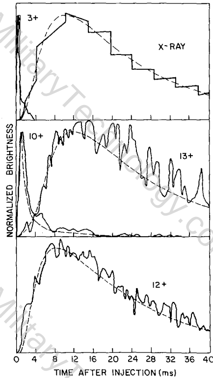
FIG. 6. Normalized chordal brightnesses from different ionization states of injected silicon. The dashed curves are predictions from the computer model.
