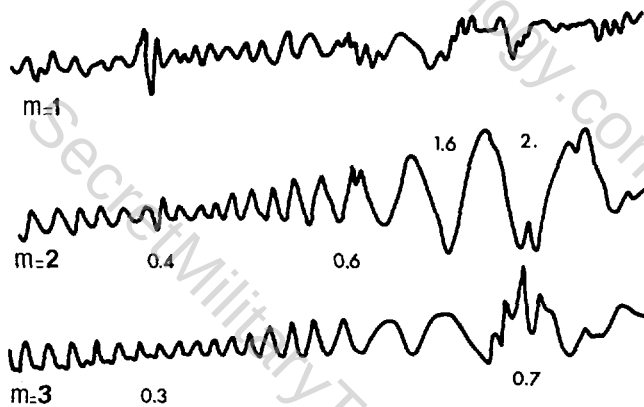
FIG.1. Oscillatory behaviour of m = 2 , n = 1 toroidal mode, including its two neighbouring satellites. Numbers refer to island size just before disruption.
