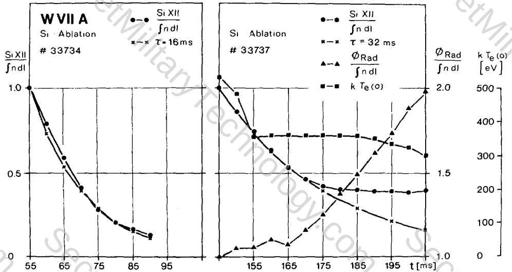
FIG.12. Decay of Si XII/fndI signals after ablation (time of ablation 50 ms and 140 ms). Exponential decay curves are given for comparison. Central radiation \phi_{rad}/fndI from USX diodes and kT_e(0) are shown as a function of time.
