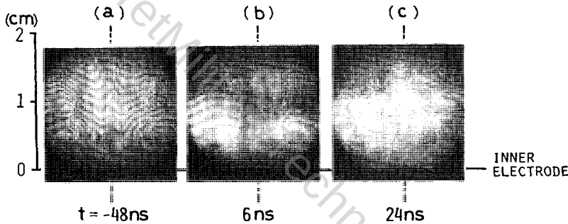
FIG. 5. A typical example of interferograms in the framing mode obtained with device C. Discharge voltage, 15 kV; working gas, 2.5 torr D_2 .
