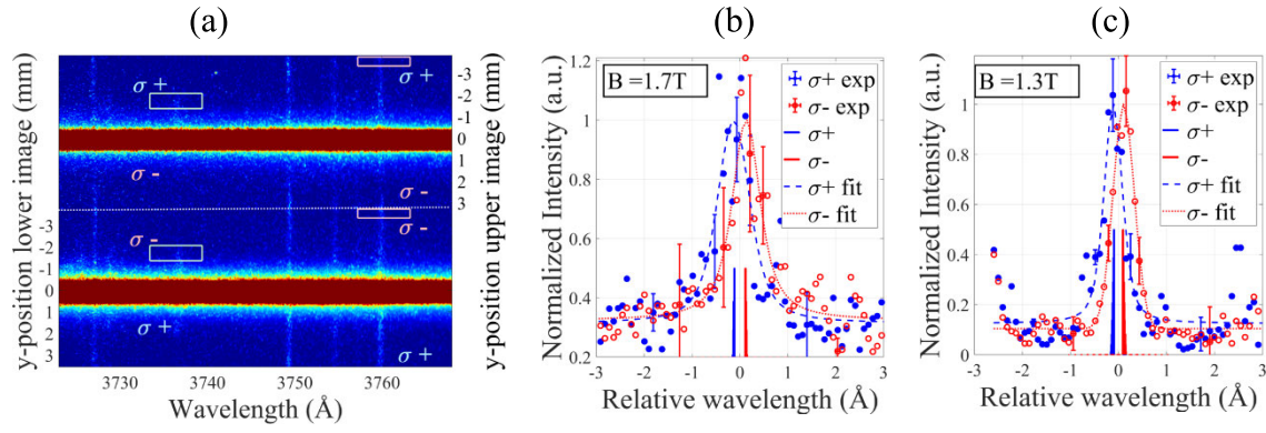
Fig. 10. (a) Spectral image of the chordally integrated spectrum of the small-scale Z-pinch at stagnation. (b) Line shapes of the O IV 3p-3d transition at 3736.85 Å, recorded at different polarizations ( \sigma^+ and \sigma^- at the upper and lower part of the detector, respectively), obtained from the lineout of the spectral image taken from r = (-1.90 \pm 0.35) mm (marked by the white rectangles), together with the best fits. The peak separation between the \sigma^+ and \sigma^- yields B = 1.7 T. The zero-density, Doppler-free Zeeman pattern is plotted at the bottom. (c) Same as (b) for the O III 3s-3p transition at 3759.87 Å, yielding B = 1.3 T at r = (-3.55 \pm 0.21) mm.
