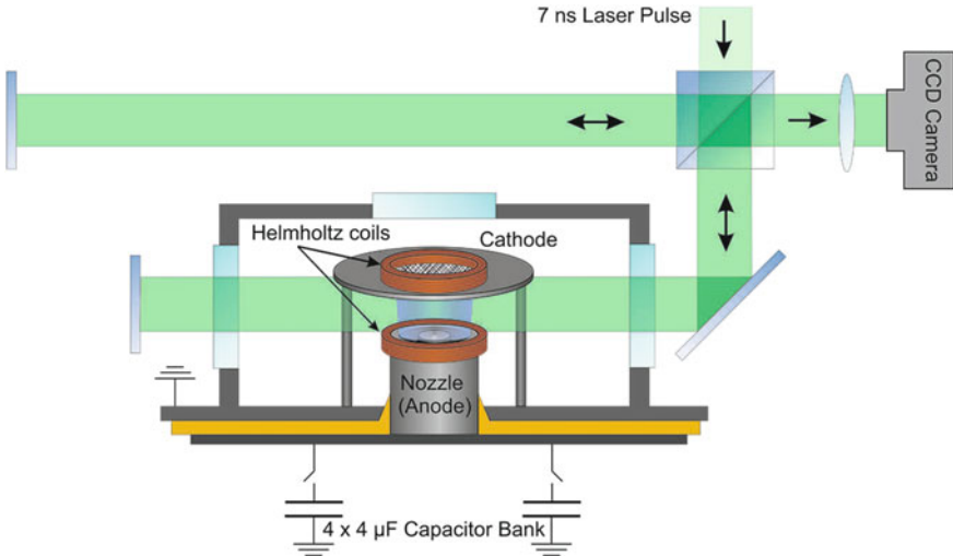
Fig. 2.7 Interferometric setup
