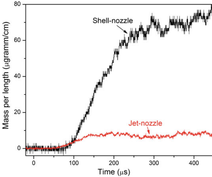
Fig. 2.11 \text{CO}_2 gas mass-per-length evolution at a distance of 5 mm from the nozzle outlet. The black curve represents the mass per length time dependence of the shell-puff. The red curve represents the mass per length time dependence of the jet-puff
