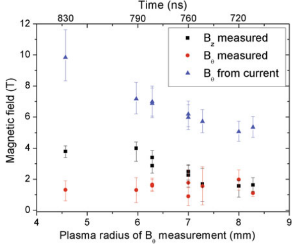
Fig. 3.8 Measured B_\theta (red dots) and B_z (black squares) as a function of the argon plasma radius measured at z = 3.5 mm from the anode for B_{z0} = 0.4 T, together with the calculated B_\theta (blue triangles) using total current and plasma radius. The upper scale shows the typical times that correspond to each plasma radius
