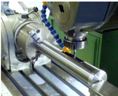
Figure 3: Photograph of the manufacturing of the movable electrode of the Einzel lens.
