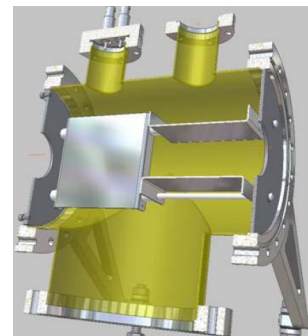
Figure 4: Beam steerers in the low injector.
