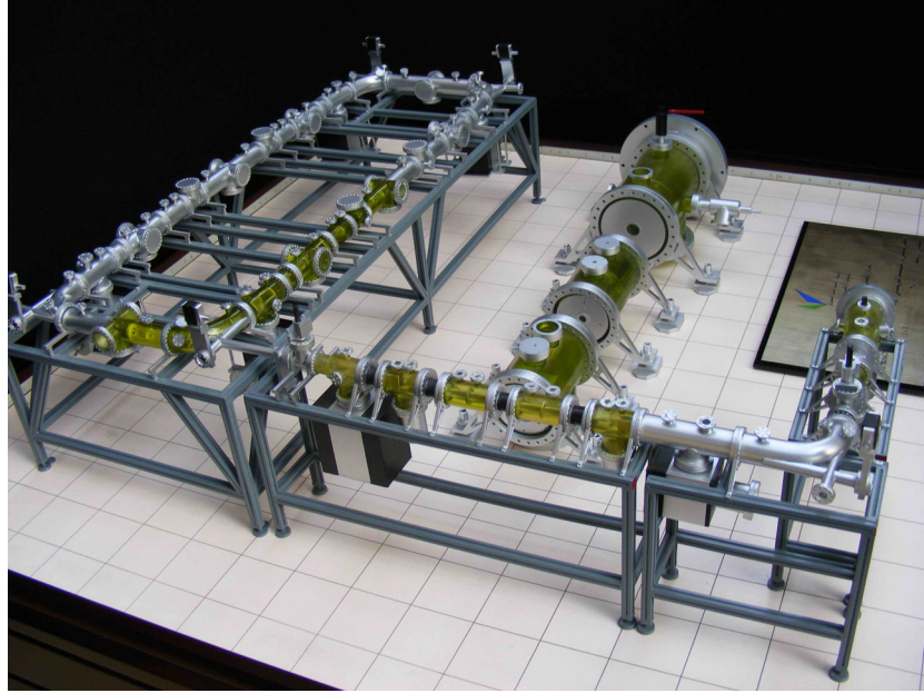
Figure 5: Illustration of the low energy complex at KACST.
