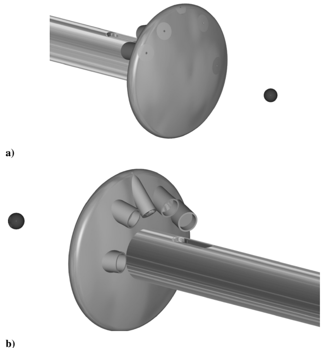
Fig. 7 Double Apollo disk model with a) front and b) rearviews showing the position of the instrumentation: ●, position of the laser focal point.
