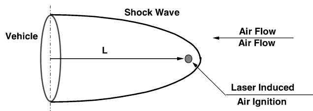
Fig. 2 Schematic of the DEAS concept.
