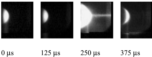
Fig. 12 Time history of the generation and extinction of the laser-supported DEAS in high-enthalpy flow.
