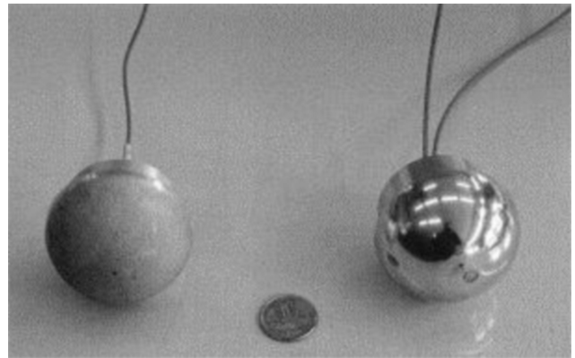
Fig. 6 Hemisphere-cylinder models.
