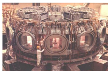
Figure 7. The T-15 superconducting tokamak.
