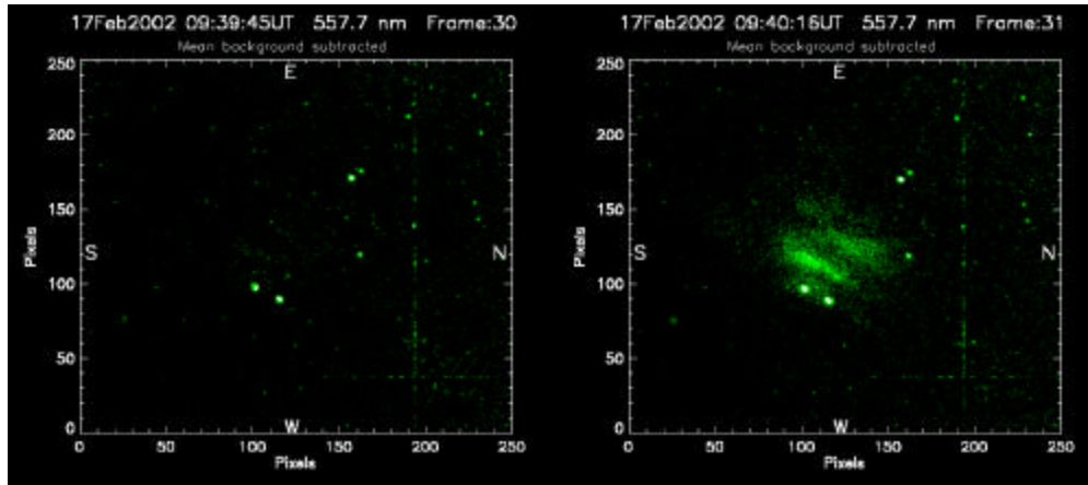
Fig. 4. Optical emission at 5577 Å produced at the HAARP Gakona Facility during the February optical campaign detected using the NRL imager.
