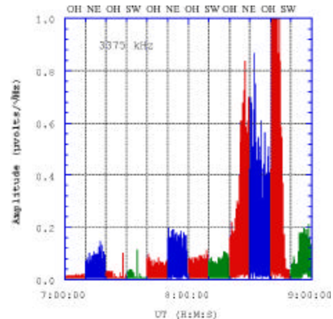
Fig. 3. Detection of the HAARP HF transmitter at 15 - 17 Re using the WIND spacecraft.
