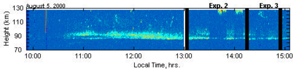
Fig. 2. Detection of Polar Mesospheric Summer Echoes using the HAARP HF transmitter in the radar mode.
