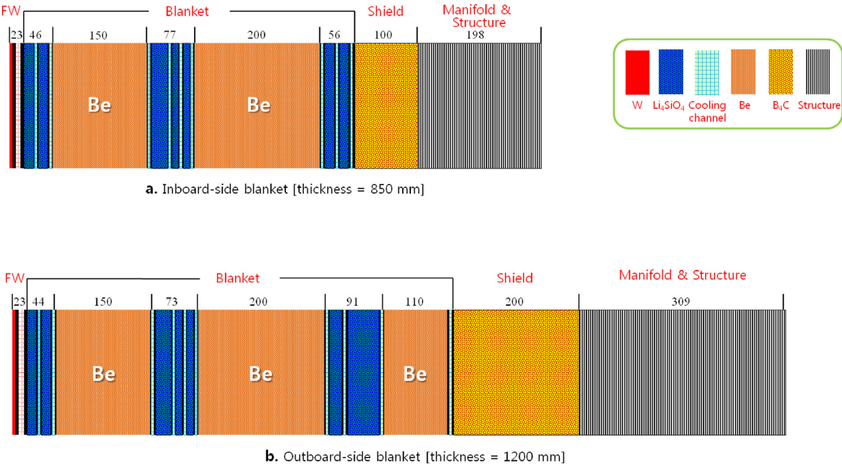
Fig. 3. Assumption for the thickness of inboard and outboard-side blankets (unit: mm).
