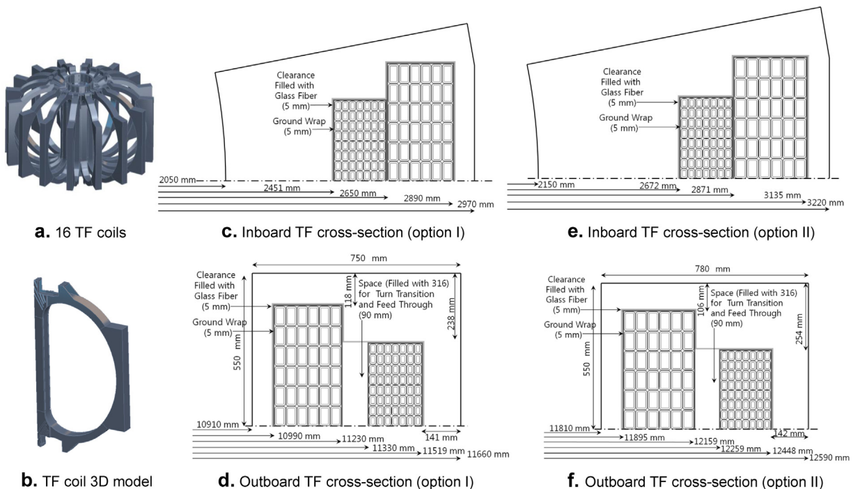
Fig. 1. A preliminary 3D modeling for TF coils (a, b) and detailed inboard and outboard TF magnet cross-sections for both option I and II (c–f).
