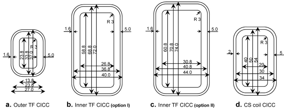
Fig. 2. Physical dimensions of the assumed CICC (unit: mm).
