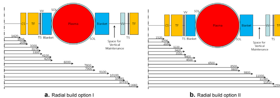
Fig. 4. Radial build of K-DEMO option I and II (unit: mm).
