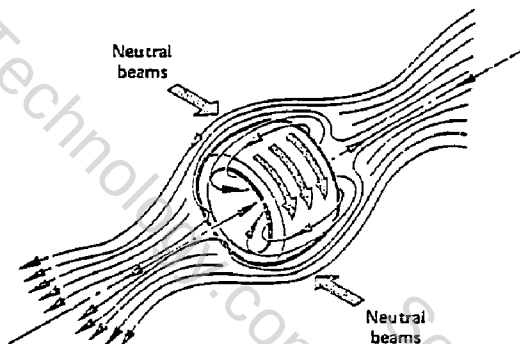
Fig. 2. Neutral-beam-driven field-reversed mirror machine.
