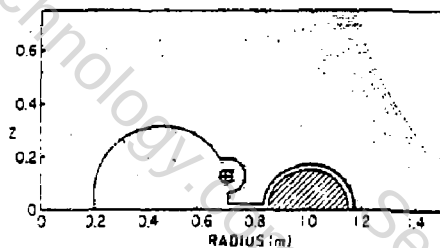
Figure 1. Vacuum field for S-1 in holomak-mode operation. Hexapole null, for start-up, is placed at R=0.575 , Z=0 . Equilibrium coils: I_E=393,000 amperes @ R=1.5 , Z=0.825 ; Nulling coils: I_N=85,370 amperes @ R=0.7 , Z=0.125 . (PPPL-79245)
