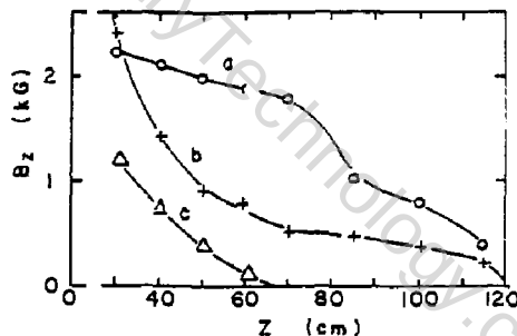
Fig. 1. B_z in the flux conserver at 10 \mu s after the voltage is applied to the gun for initial magnetic fields of a) 4.5 kG, b) 10 kG and c) 19 kG inside the inner electrode of the gun.
