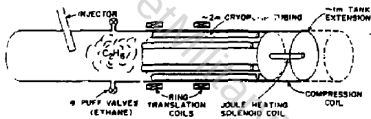
Fig. 2. Recent Changes in RECE-Christa for Plasma Confinement Experiments
