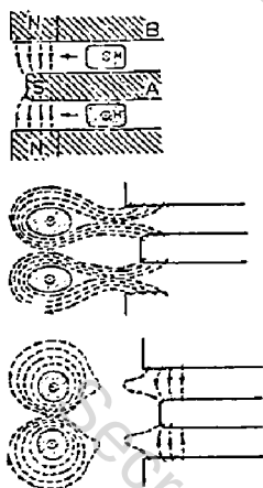
Fig. 1. Spheromak generation, using a coaxial plasma gun with poloidal field at the muzzle.
