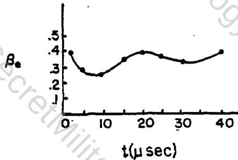
Figure 3 Time dependence of \beta_e . At 40 \mu\text{sec} the externally applied field has dropped to half its maximum.
