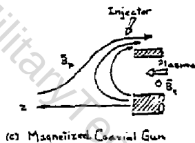
Fig. 1 (a) \psi mirror formed by 6 supported current loops and B_z . (b) \psi mirror as in (a) and (c) mirror at the nozzle of a magnetized coaxial plasma gun.
