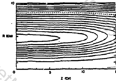
Figure 2 Contours of constant poloidal flux at 2 \mu\text{sec} after the start of the fast B_z field. The contours are calculated from magnetic field measurements made in the plasma and are plotted in intervals of 20\text{mG}\cdot\text{cm}^2 .
