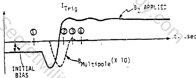
79 13-57 Figure 2. Stages of Toroid Formation Using Cusp Holdoff and Triggered Reconnection (second half-cycle operating mode)
