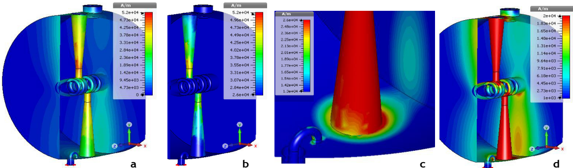
Figure 5: Critical current density (power deposition) on various scale in MEBT rebunchers for 120 kV.
