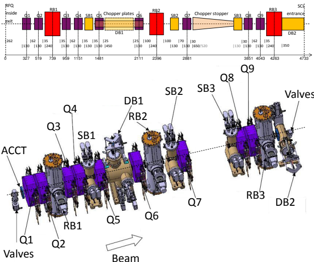
Figure 3: MEBT design.
