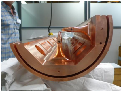
Figure 2: IPHI half-RFQ.
