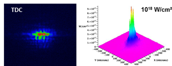
Figure 5: (Optimized) focal spot for the shot on the 25 \mu m wire with 396 J @ 3 ps and 1018 W/cm 2 .
