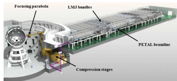
Figure 3: Implementation of PETAL laser on the LMJ facility.
