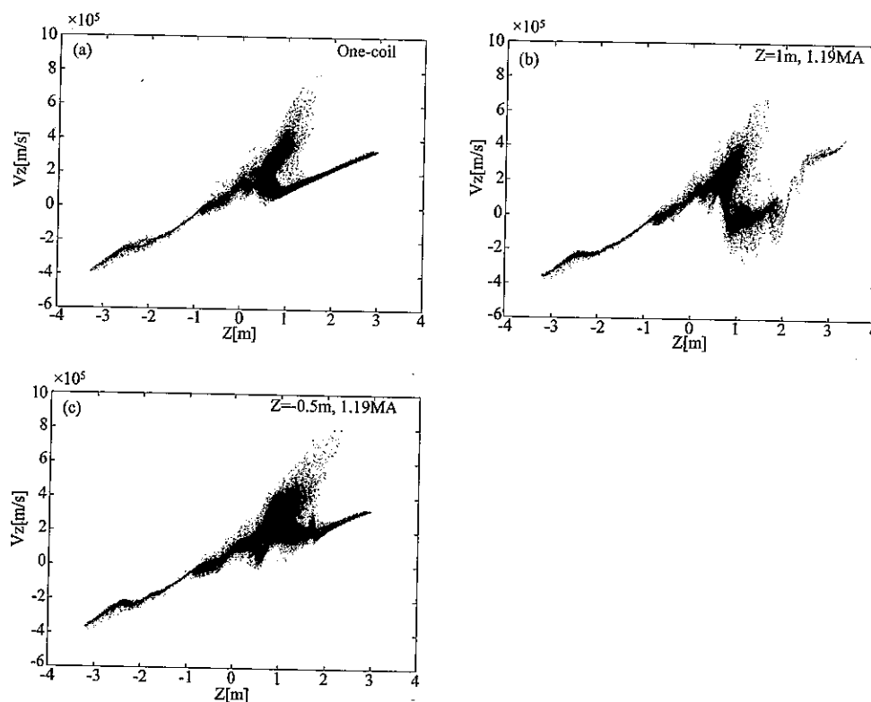
Fig. 5. Phase space of v_z : (a) one-coil case, (b) two-coil case of Z = 1.0 m and I = 1.19 MA, (c) two-coil case of Z = -0.5 m and I = 1.19 MA.
