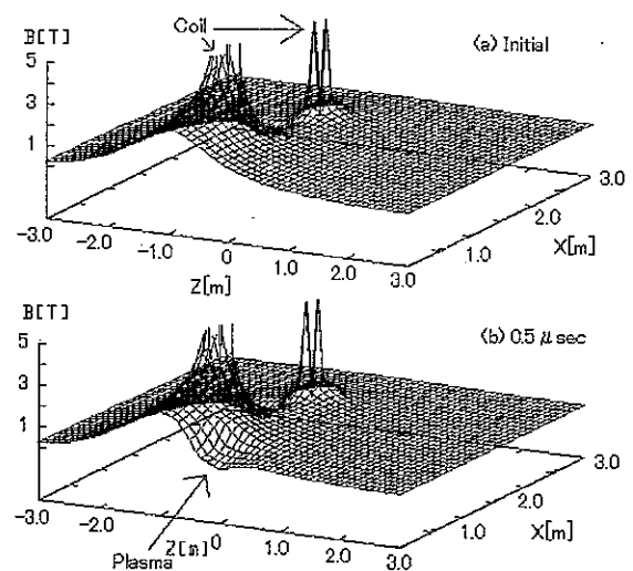
Fig. 4. Magnetic field distributions: (a) initial time, (b) 0.5 \mu\text{sec} , case of Z = -0.5 m and I = 1.19 MA.
